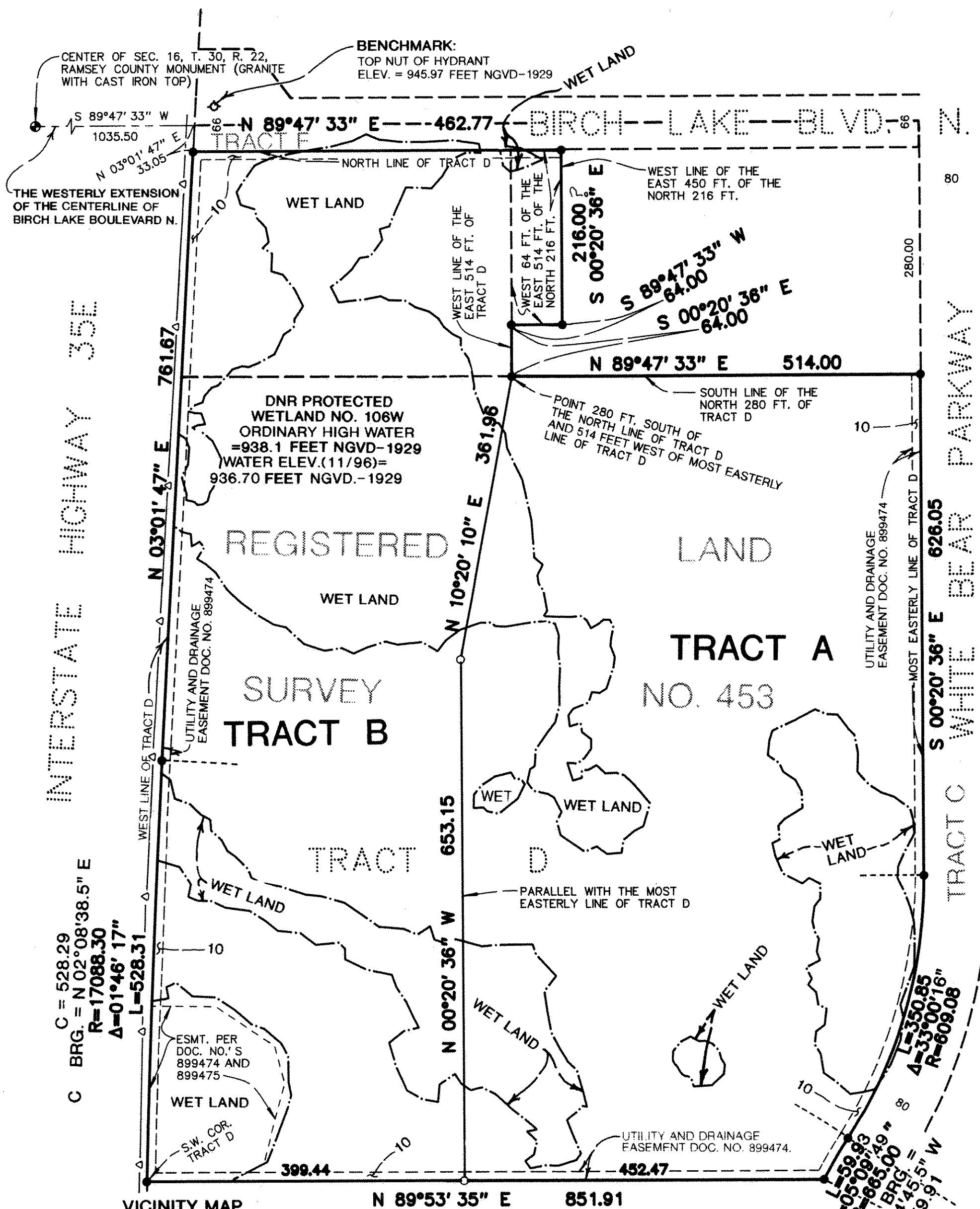
VICINITY MAP SEC. 16, T. 30, R. 22, RAMSEY COUNTY
