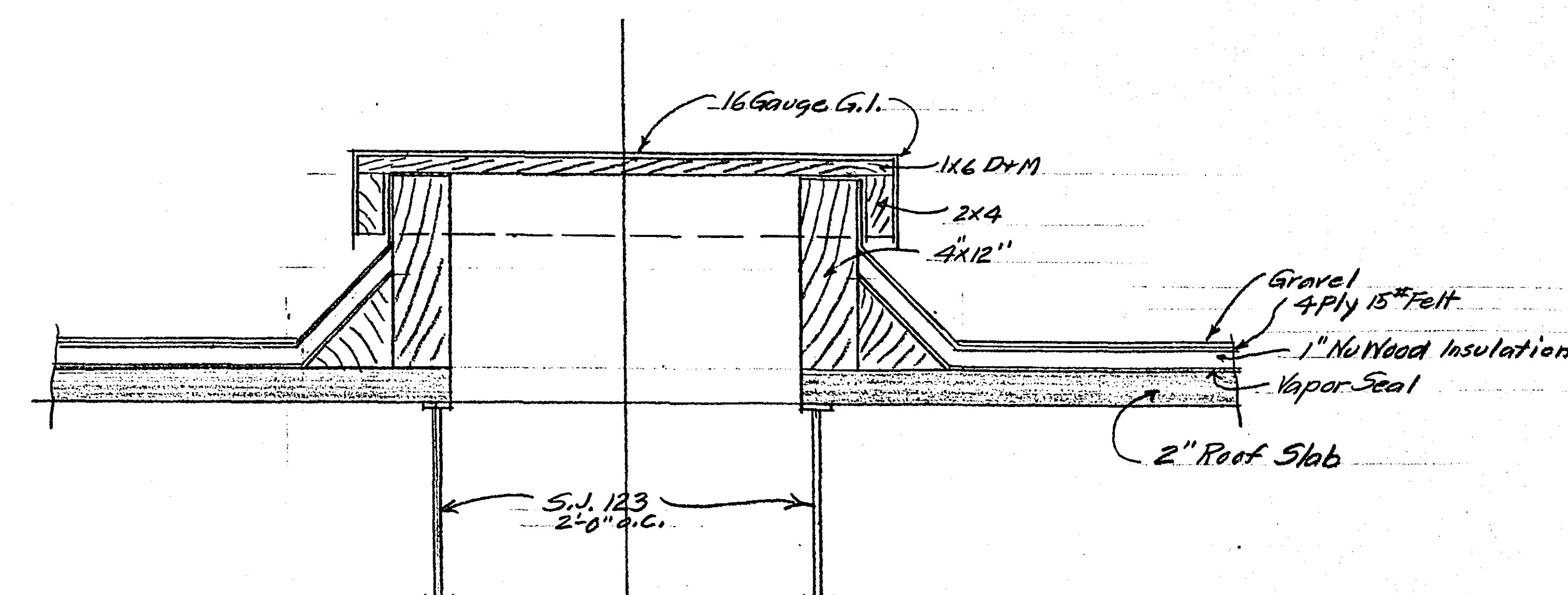
SECTION
