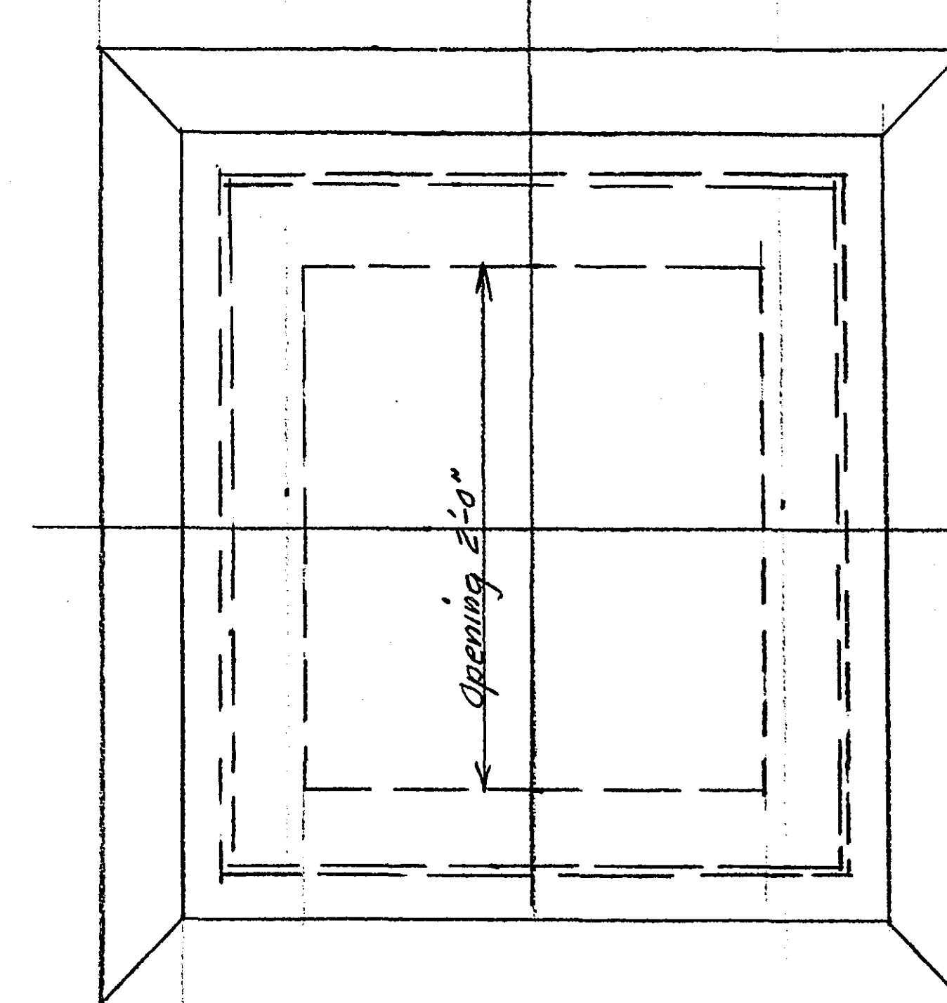
PLAN
