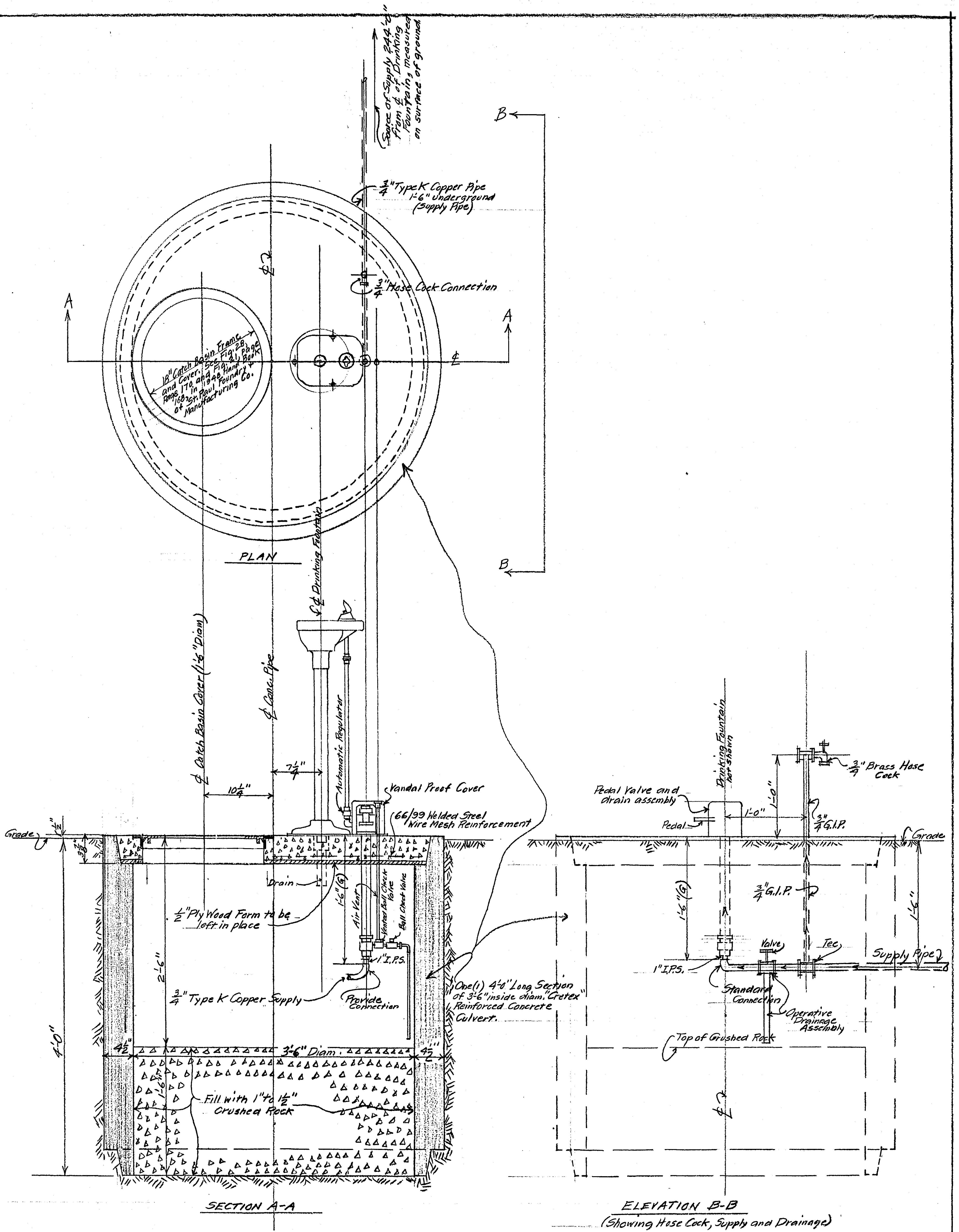
HOSE COCK AND DRINKING FOUNTAIN ASSEMBLY SCALE 1 1/2" = 1'-0"
