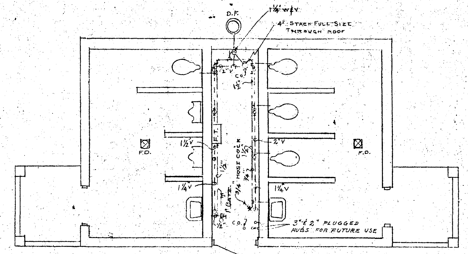
EXPOSED PIPING PLAN SCALE 1/4"=1'-0"
