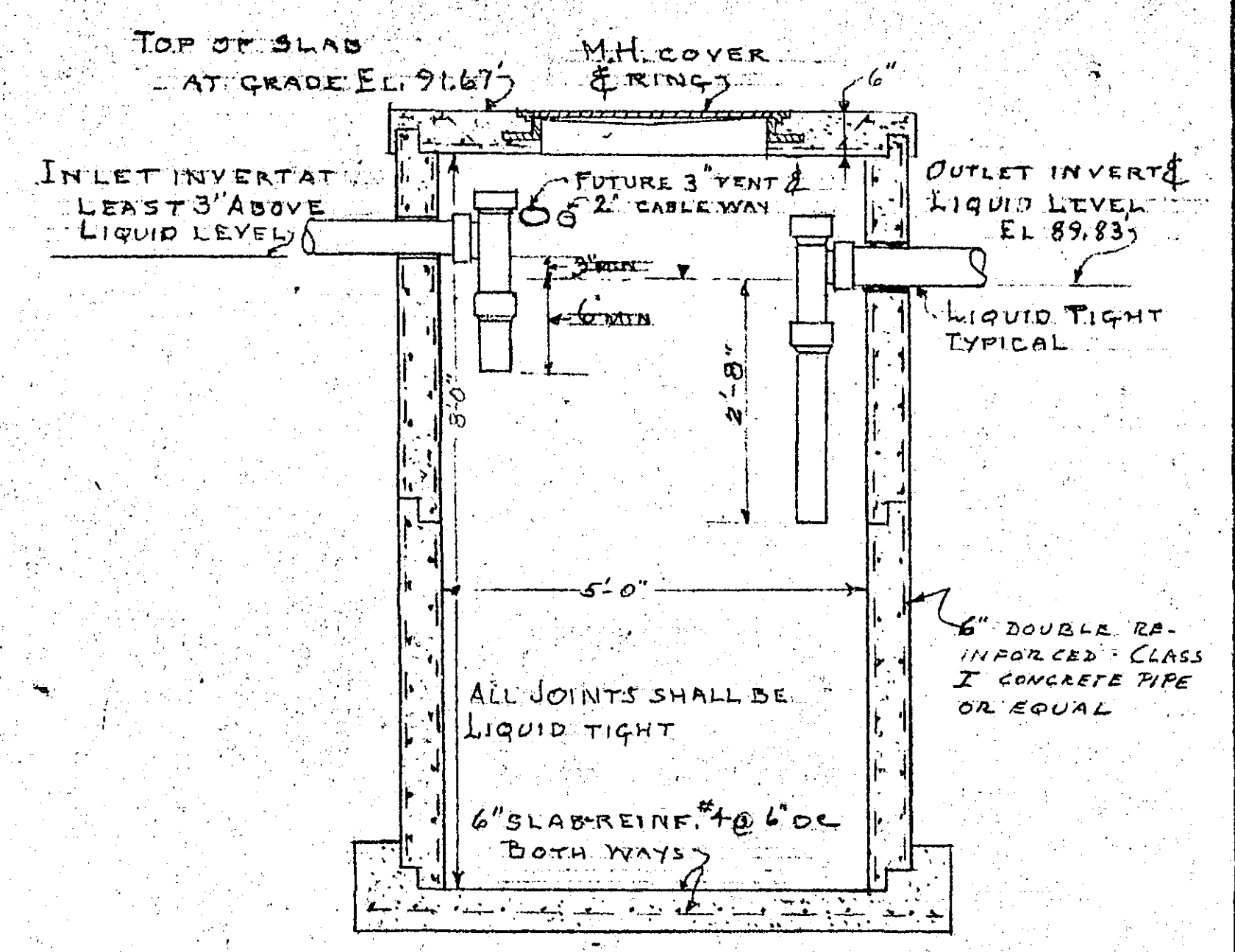
DETAIL OF SEPTIC TANK SCALE 1/2"=1'-0"
