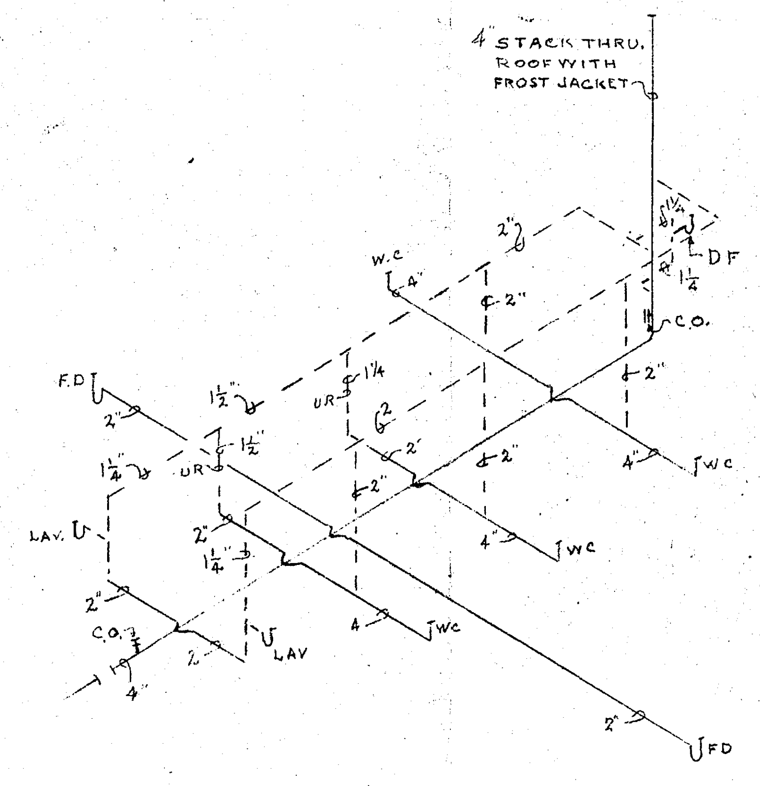
WASTE & VENT PIPING DIAGRAM NO SCALE
