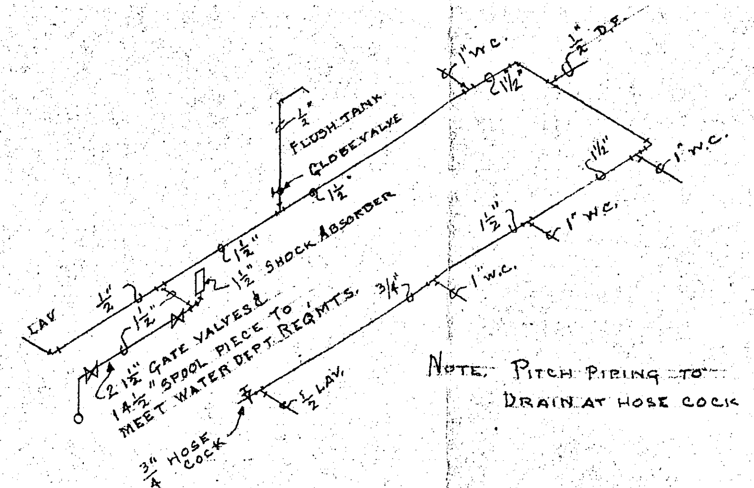
WATER PIPING DIAGRAM NO SCALE
