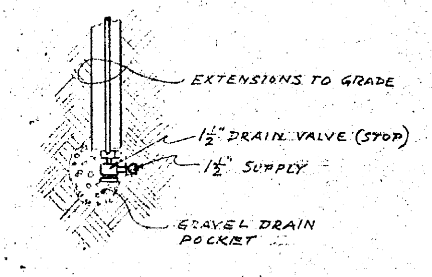
DETAIL AT DRAIN VALVE NO SCALE
