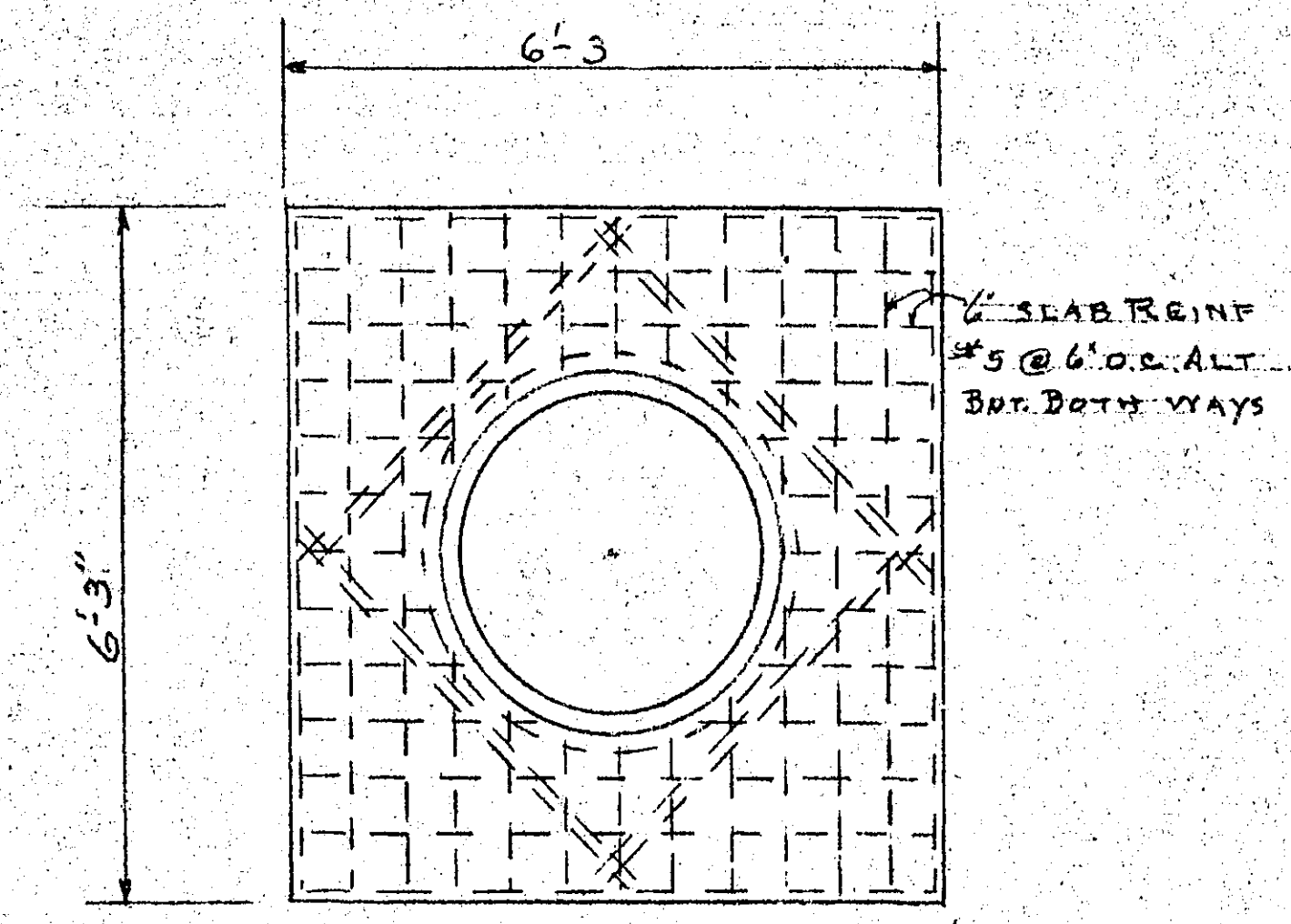
PLAN OF TOP SLAB
