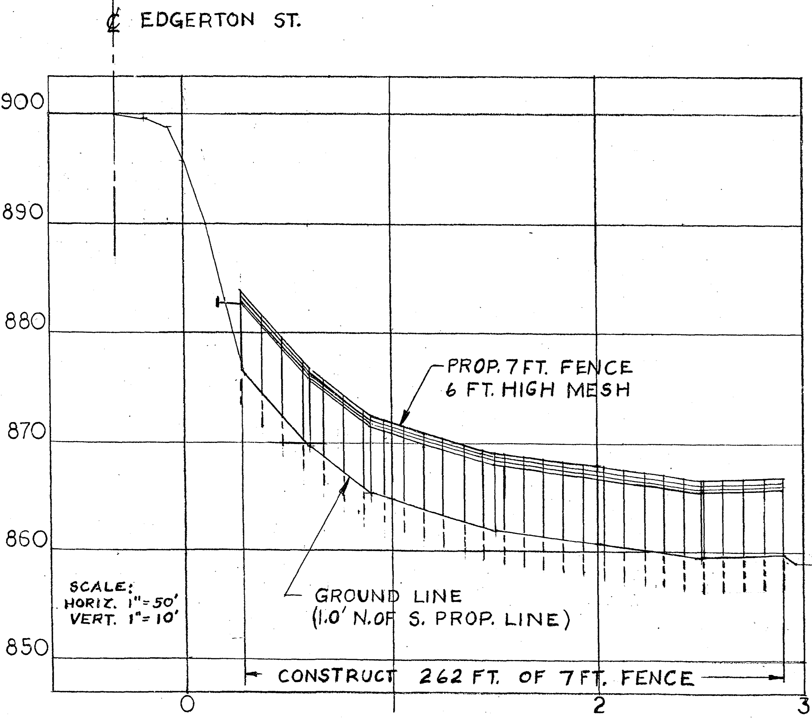
PROFILE PROPOSED FENCE
