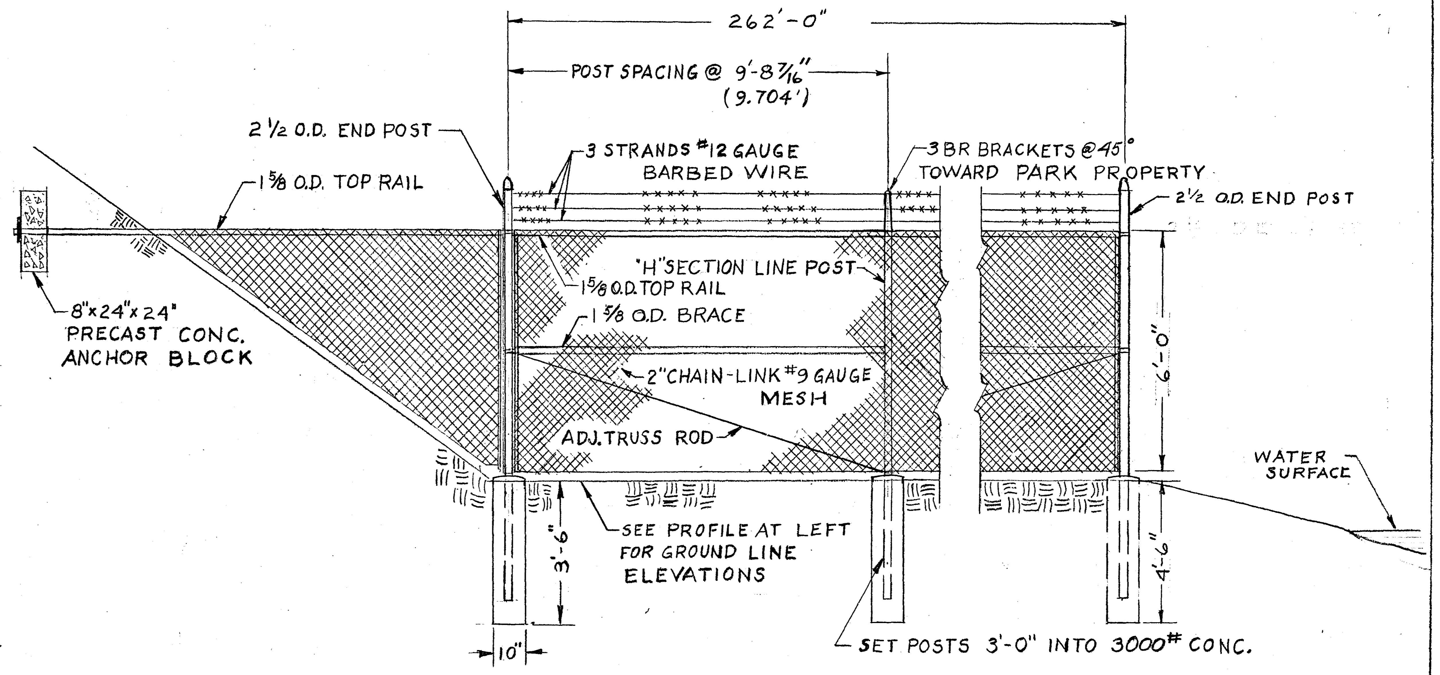
TYPICAL ELEVATION OF PROPOSED FENCE SCALE: 3/8" = 1'-0"
