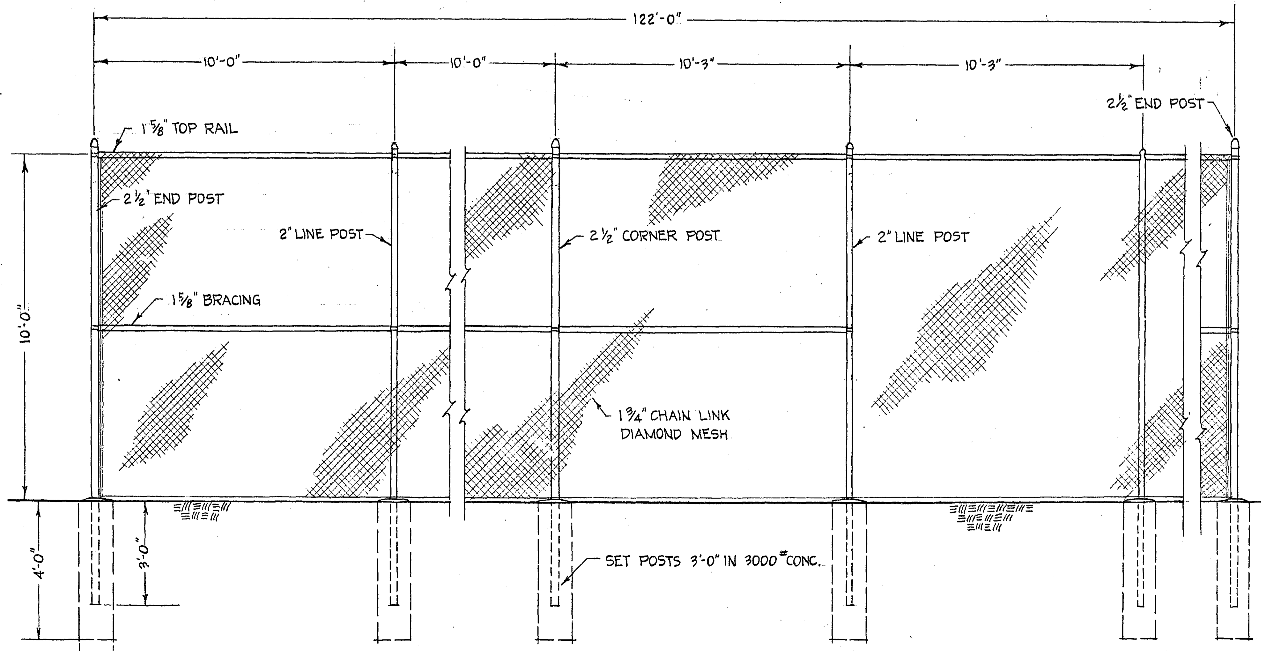
ELEVATION ON & PROP. END CLOSURE SCALE: 3/8" = 1'-0"
