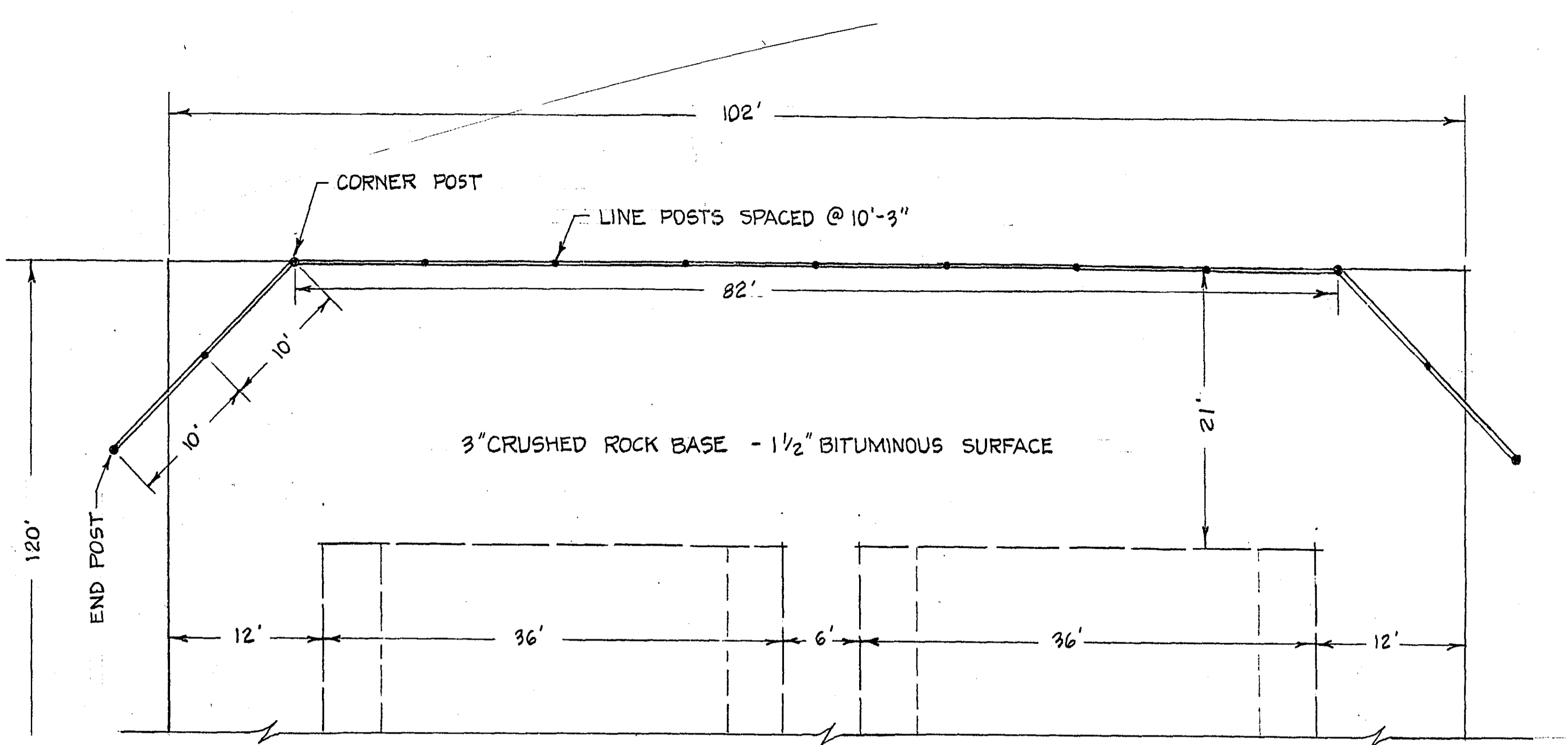
PLAN - END CLOSURE SCALE: 1" = 10'-0"
