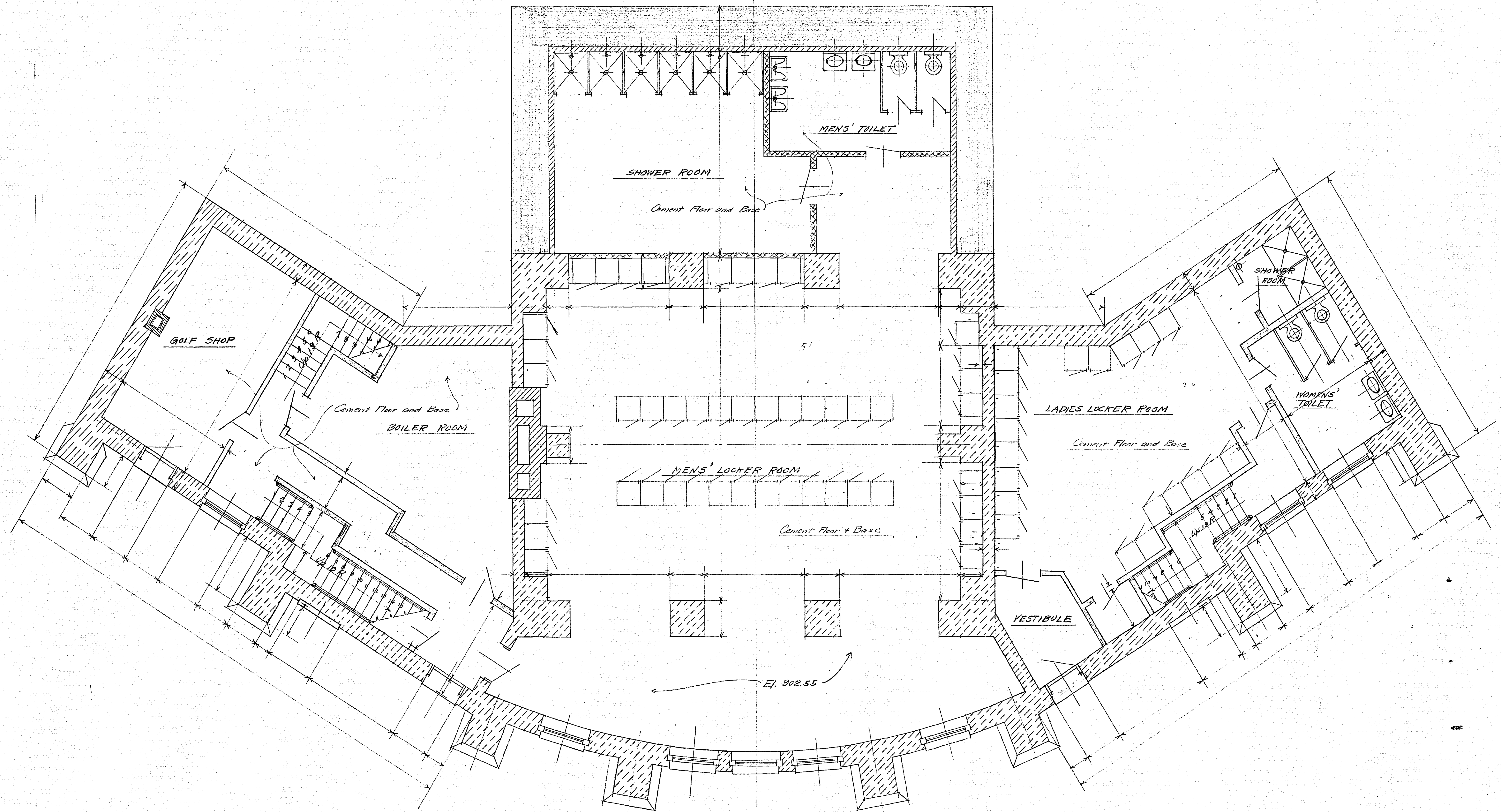
LOCKER ROOM FLOOR - \frac{1}{4}'' = 1'-0''
