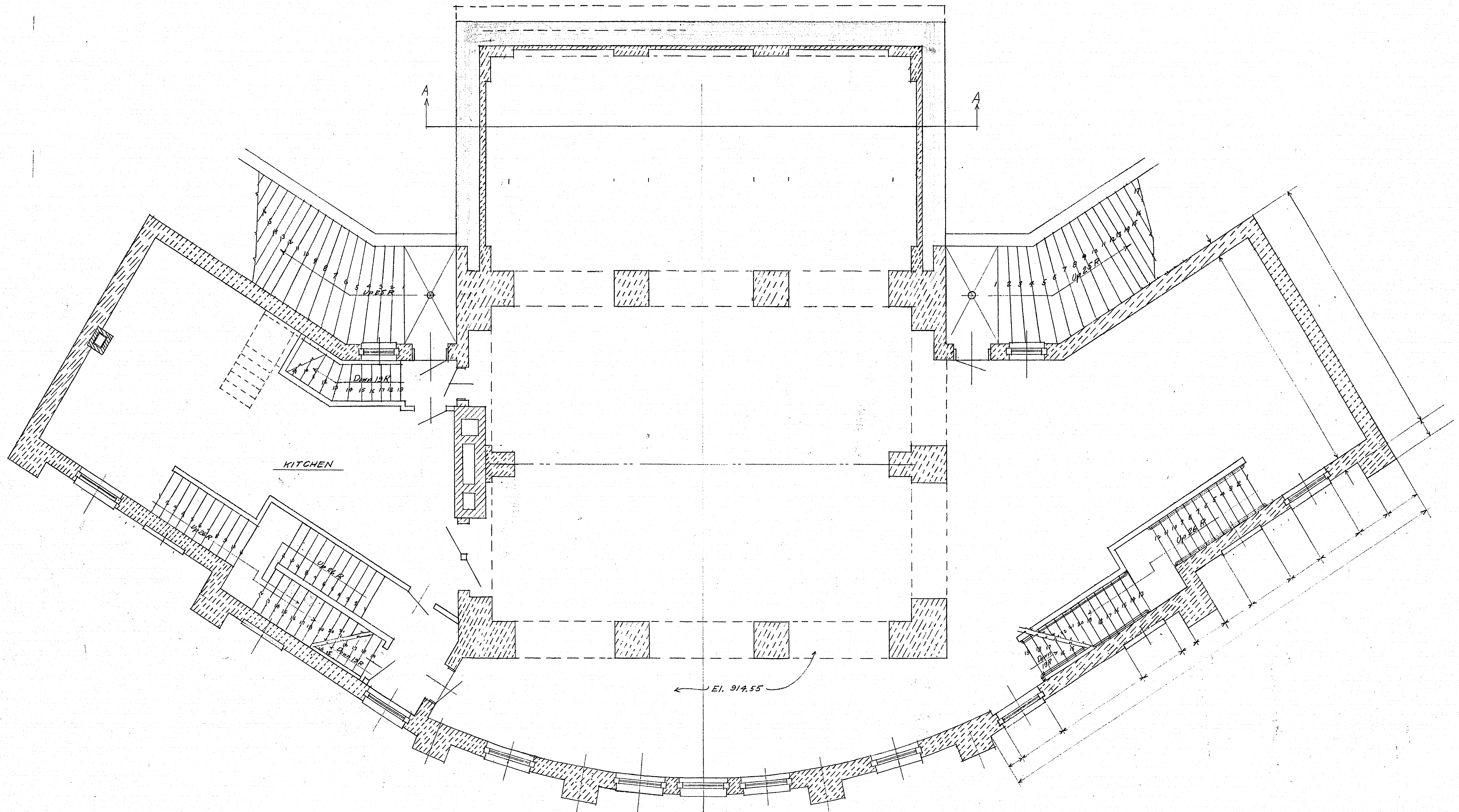
DINING ROOM FLOOR PLAN
