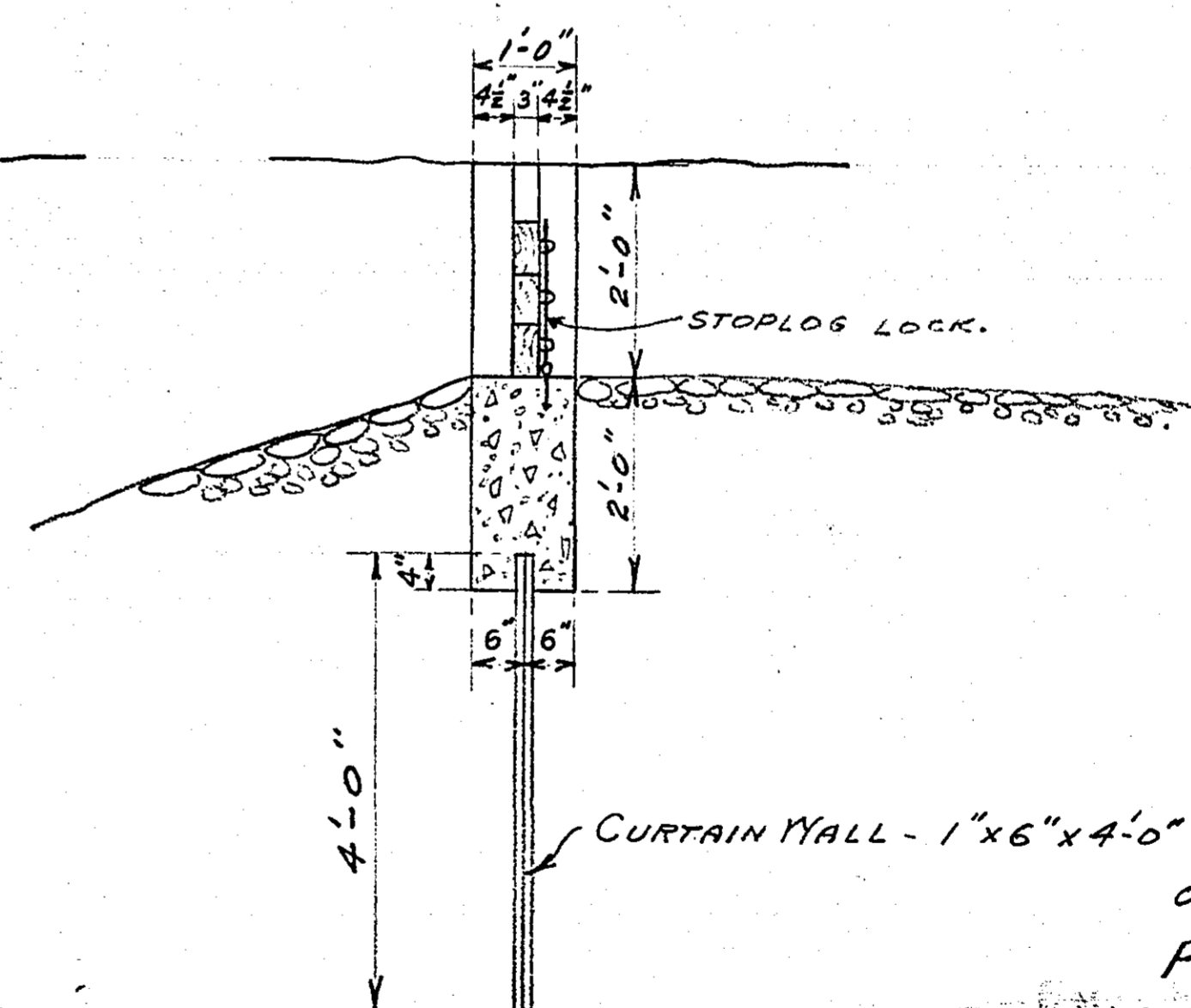
SECTION-A-A
