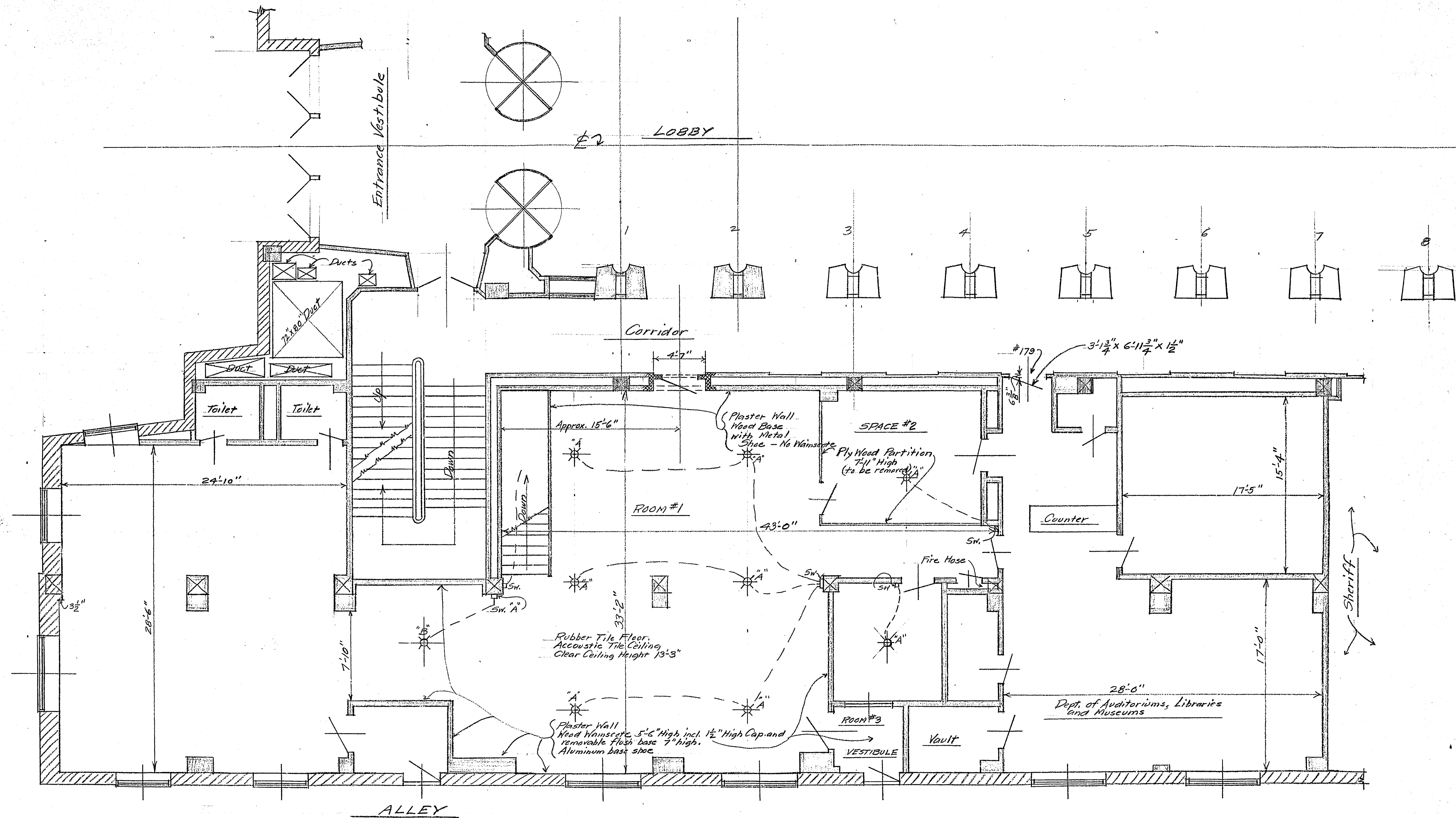
LAYOUT OF OFFICE SPACE ON N.W. CORNER OF FIRST FLOOR OF CITY HALL AND COURT HOUSE ST. PAUL, MINN SCALE \frac{1}{4}'' = 1'-0'' OCT. 1952
