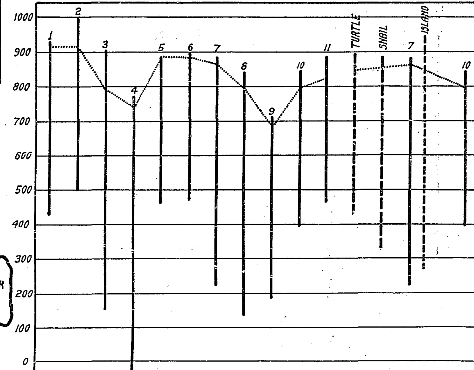
CHART SHOWING ELEVATION OF WATER TABLE IN WELLS AT VARIOUS LOCATIONS
