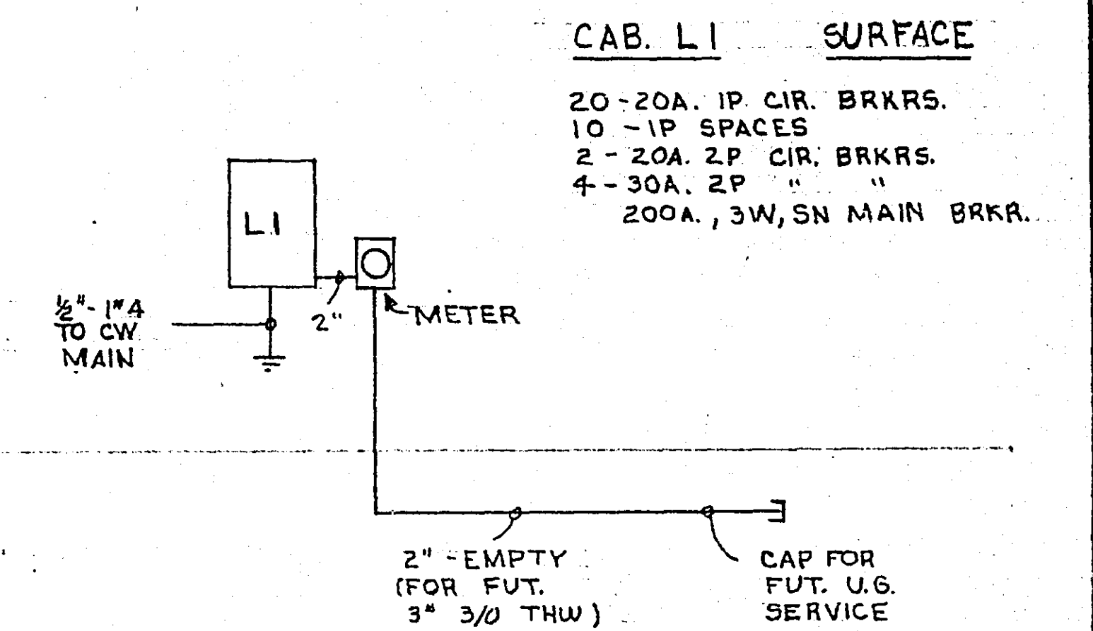
ELECTRIC RISER NO SCALE
