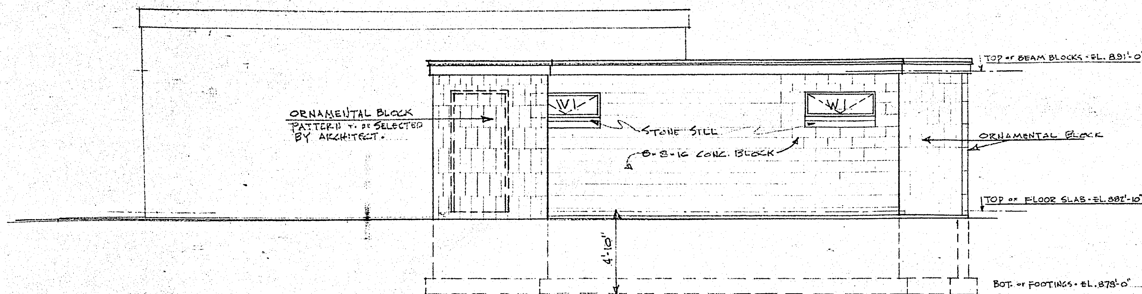
NORTH ELEVATION 1/4" = 1' - 0"
