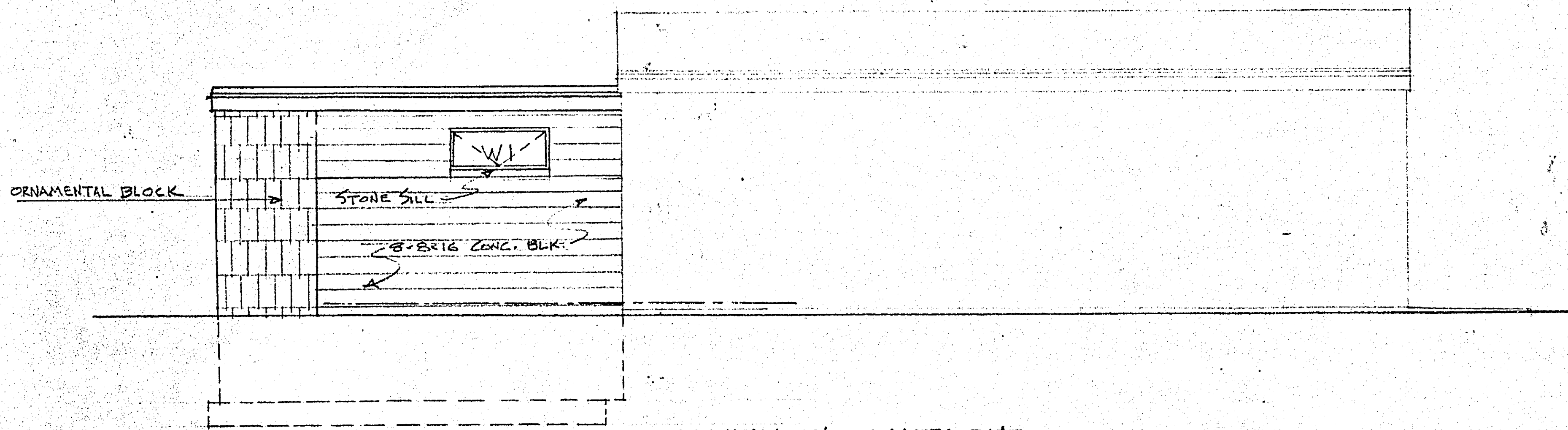
SOUTH ELEVATION 1/4" = 1' - 0"
