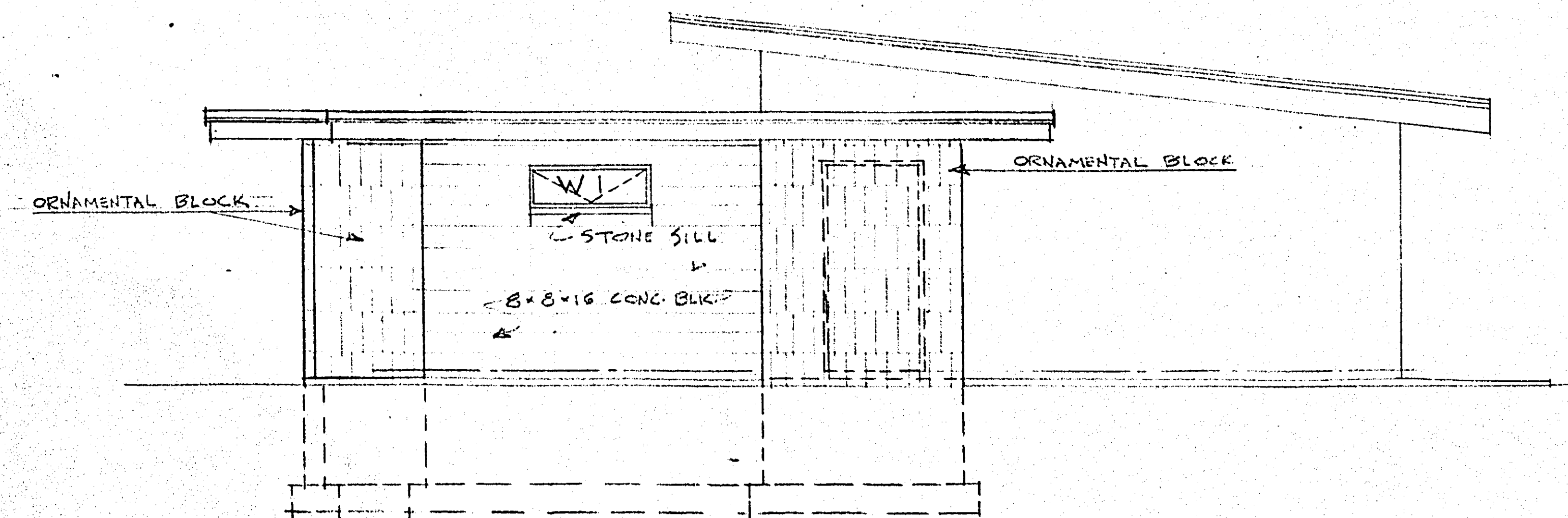
WEST ELEVATION 1/4" = 1' - 0"
