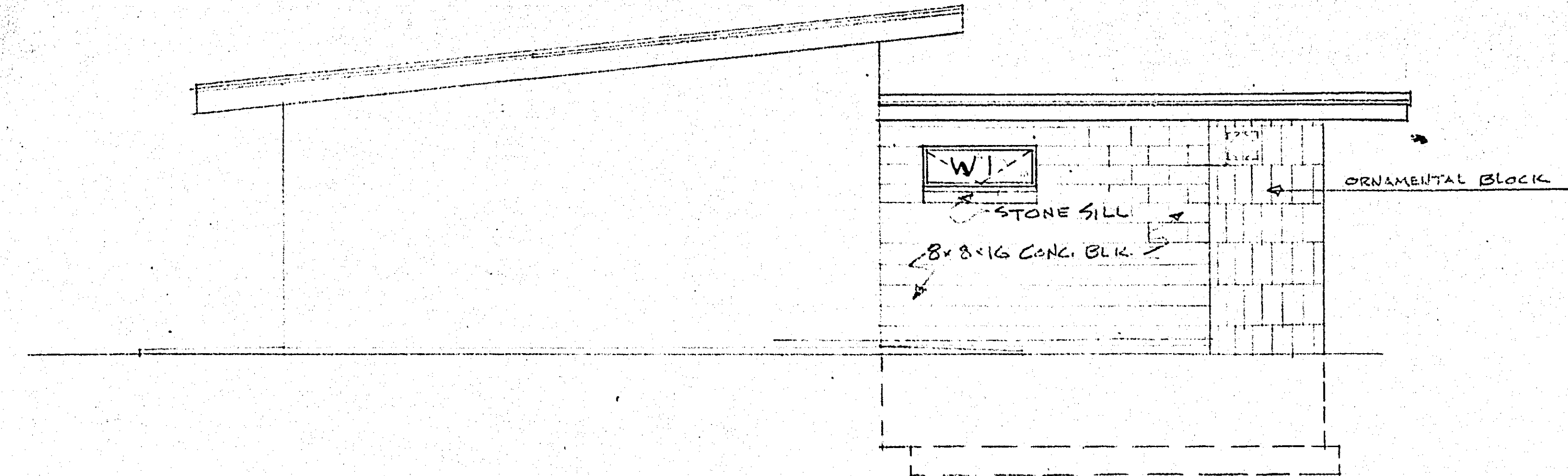
EAST ELEVATION 1/4" = 1' - 0"
