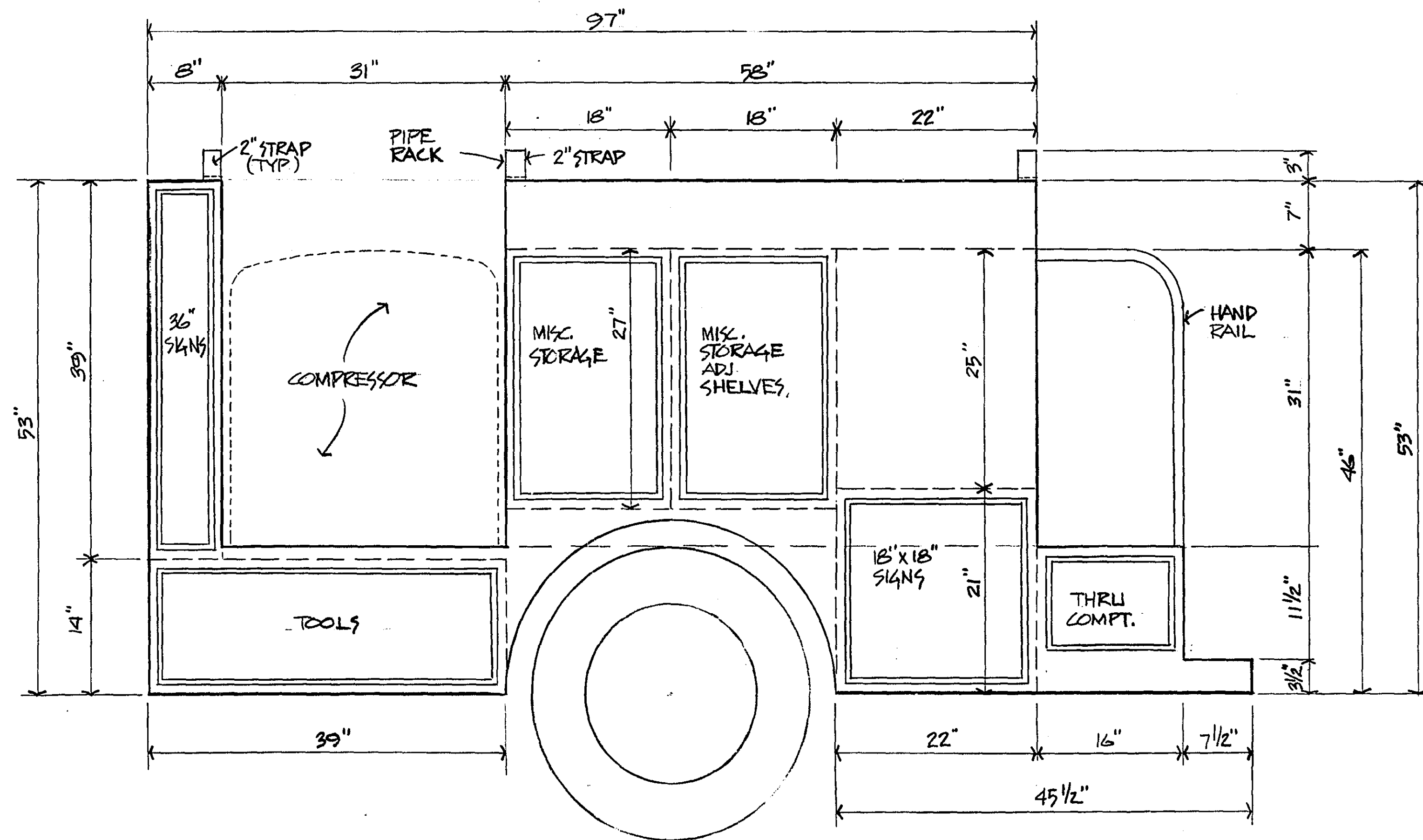
LEFT SIDE VIEW SCALE: 1"=1'-0"
