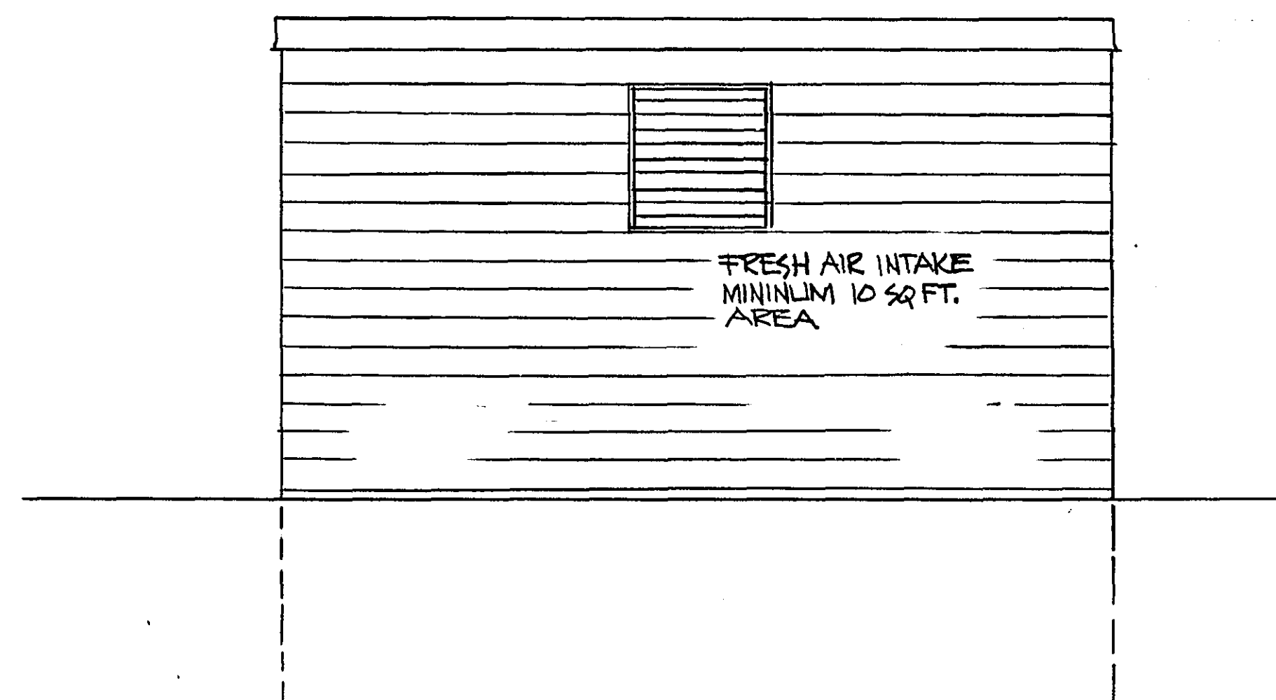
NORTHWEST ELEV. SCALE 1/4" = 1'-0"
