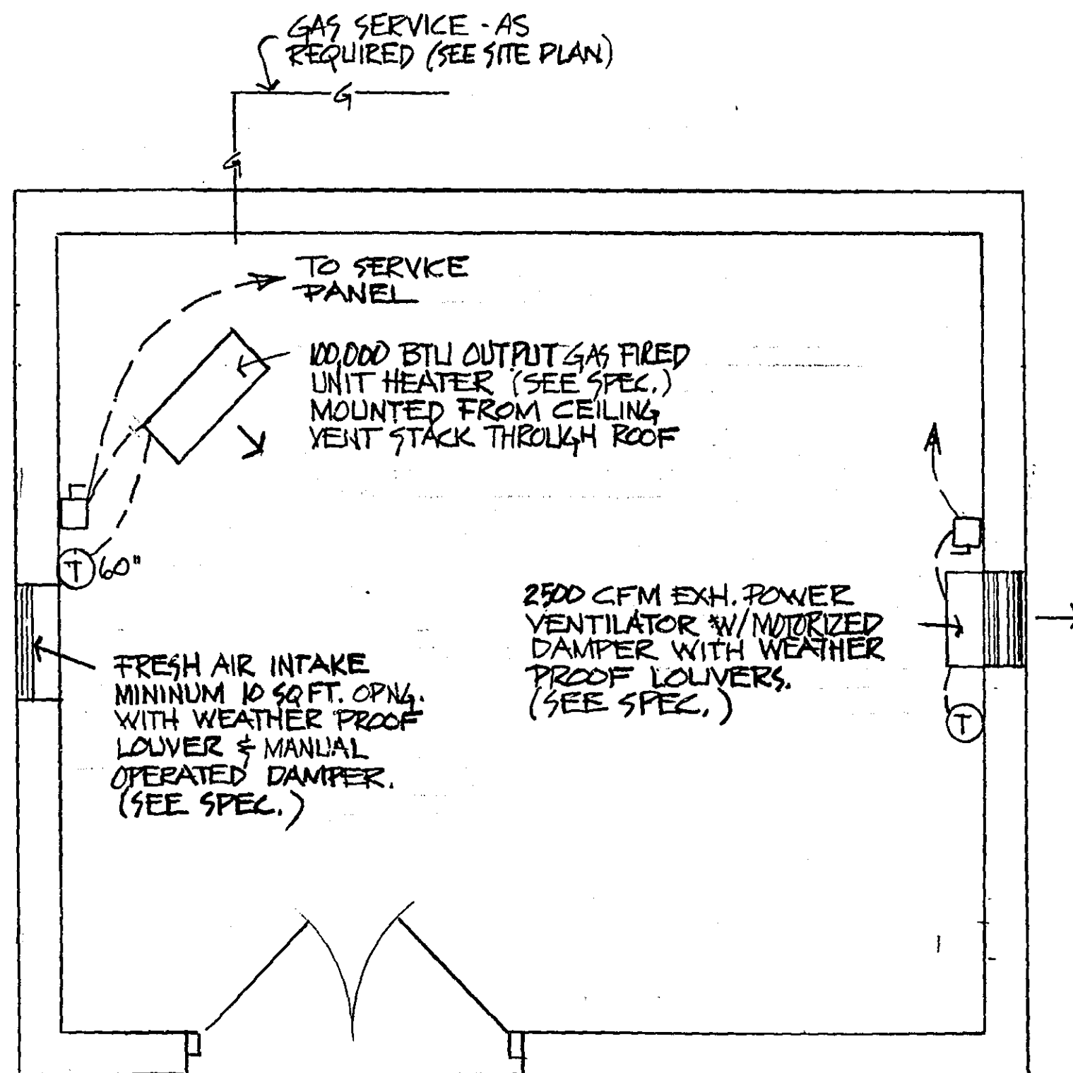
HEATING & VENTILATION PLAN SCALE: 1/4" = 1'-0"
