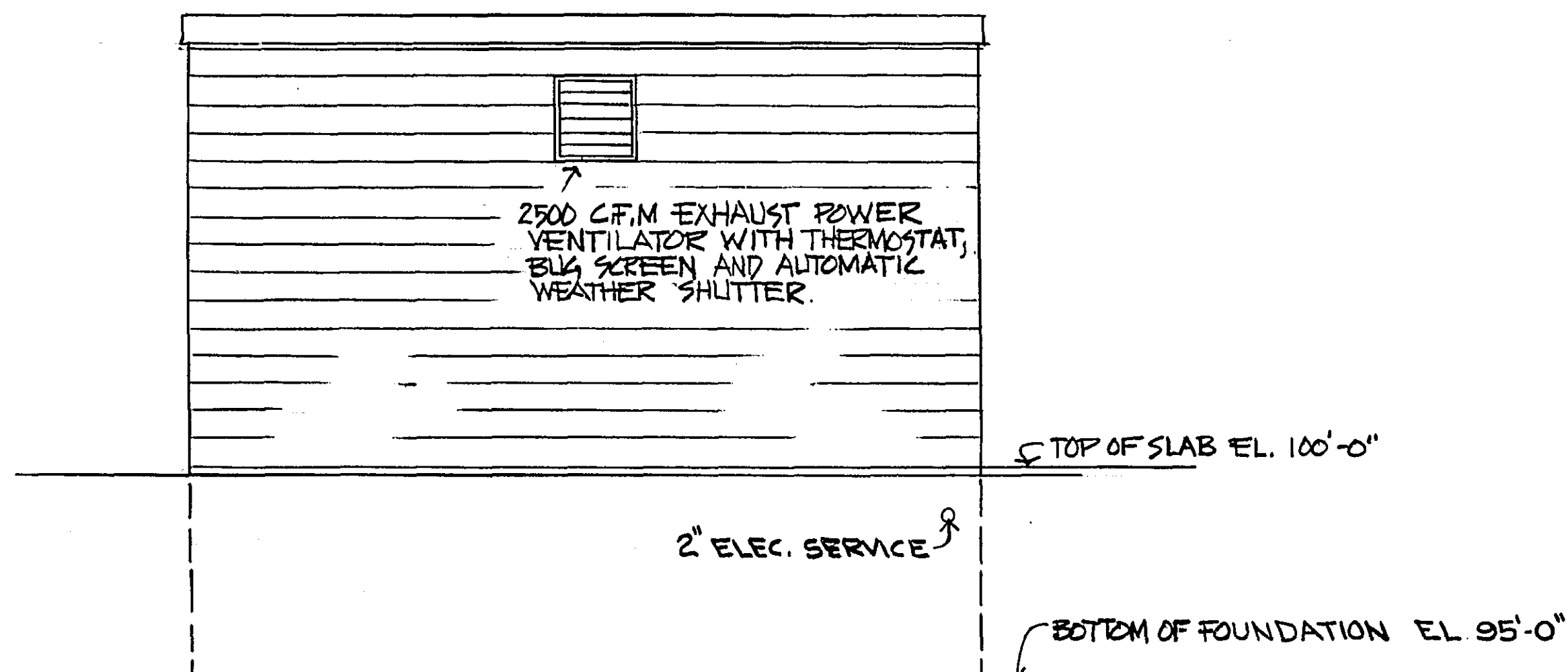
SOUTHEAST ELEV. SCALE 1/4" = 1'-0"
