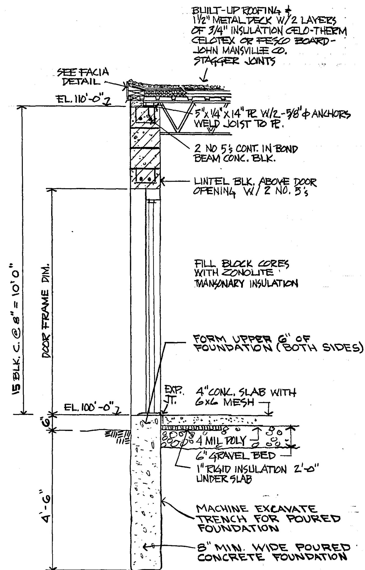
TYPICAL SECTION SCALE 1/2"=1'-0"
