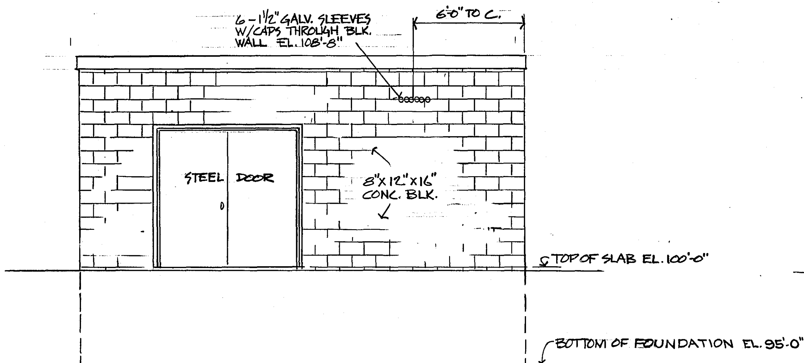
SOUTHWEST ELEV. SCALE 1/4" = 1'-0"
