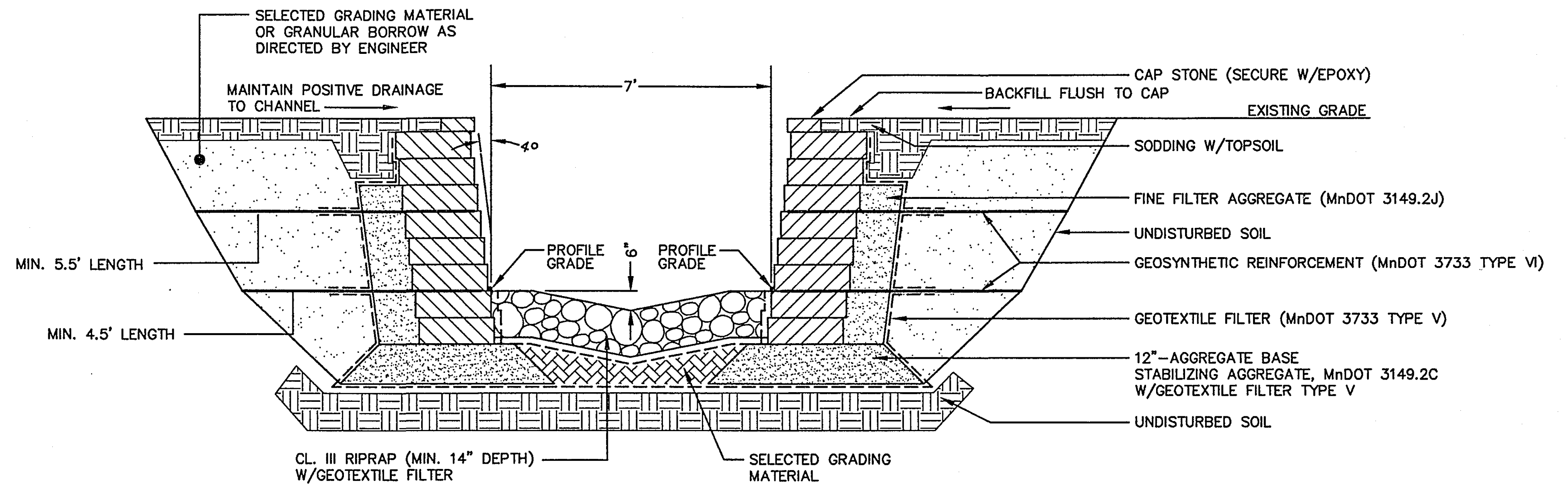
TYPICAL SECTION MODULAR BLOCK CHANNEL N.T.S.
