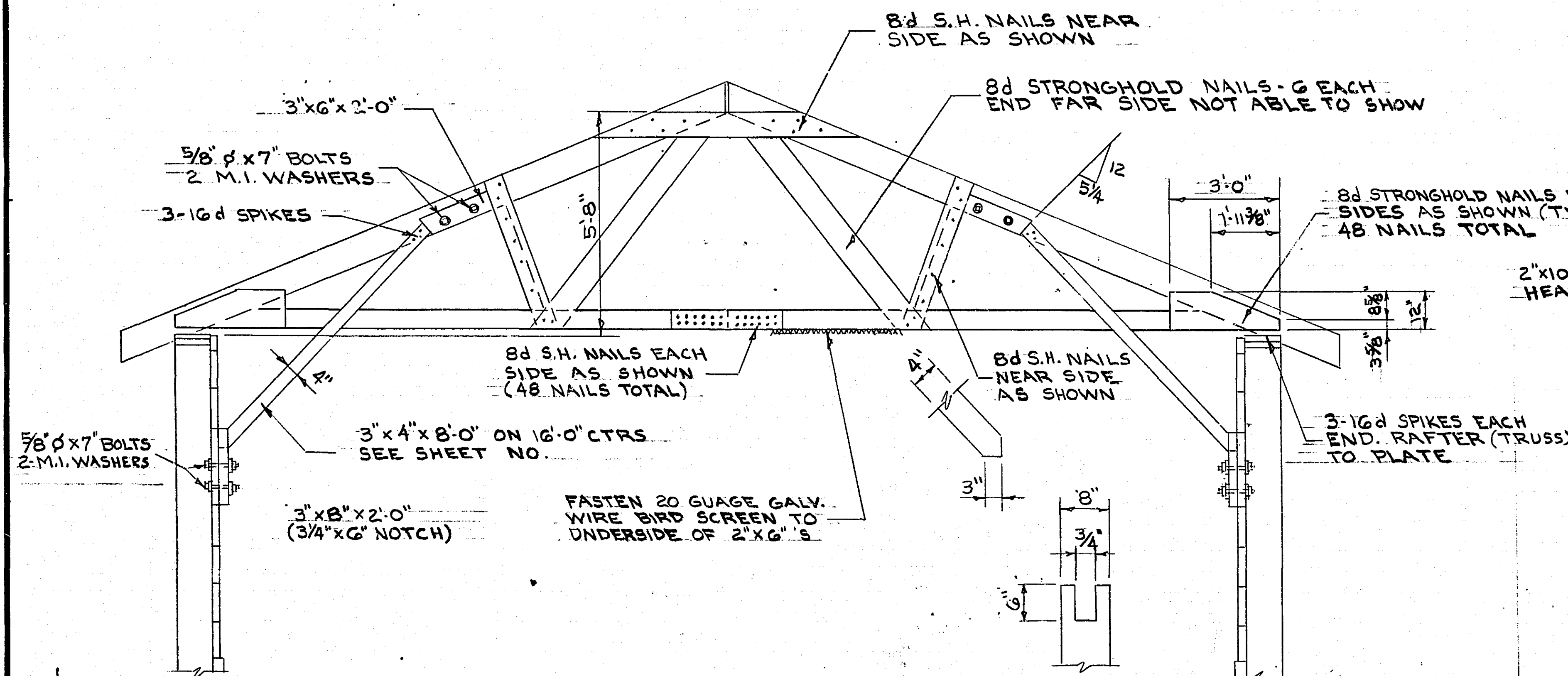
KNEE BRACE DETAIL
