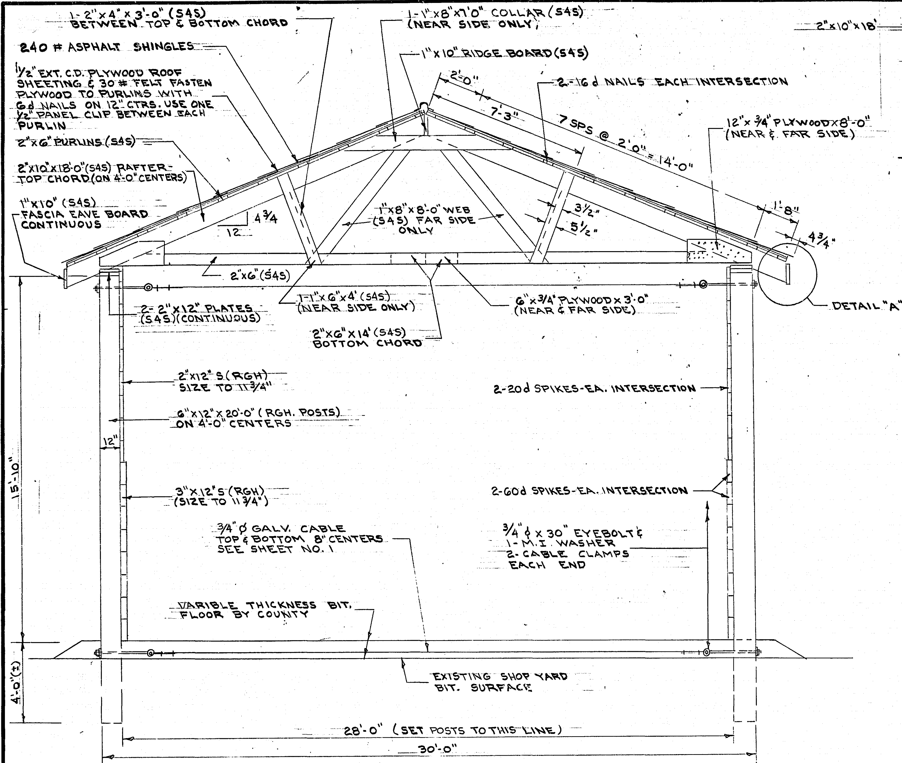
SECTION THRU SHED
