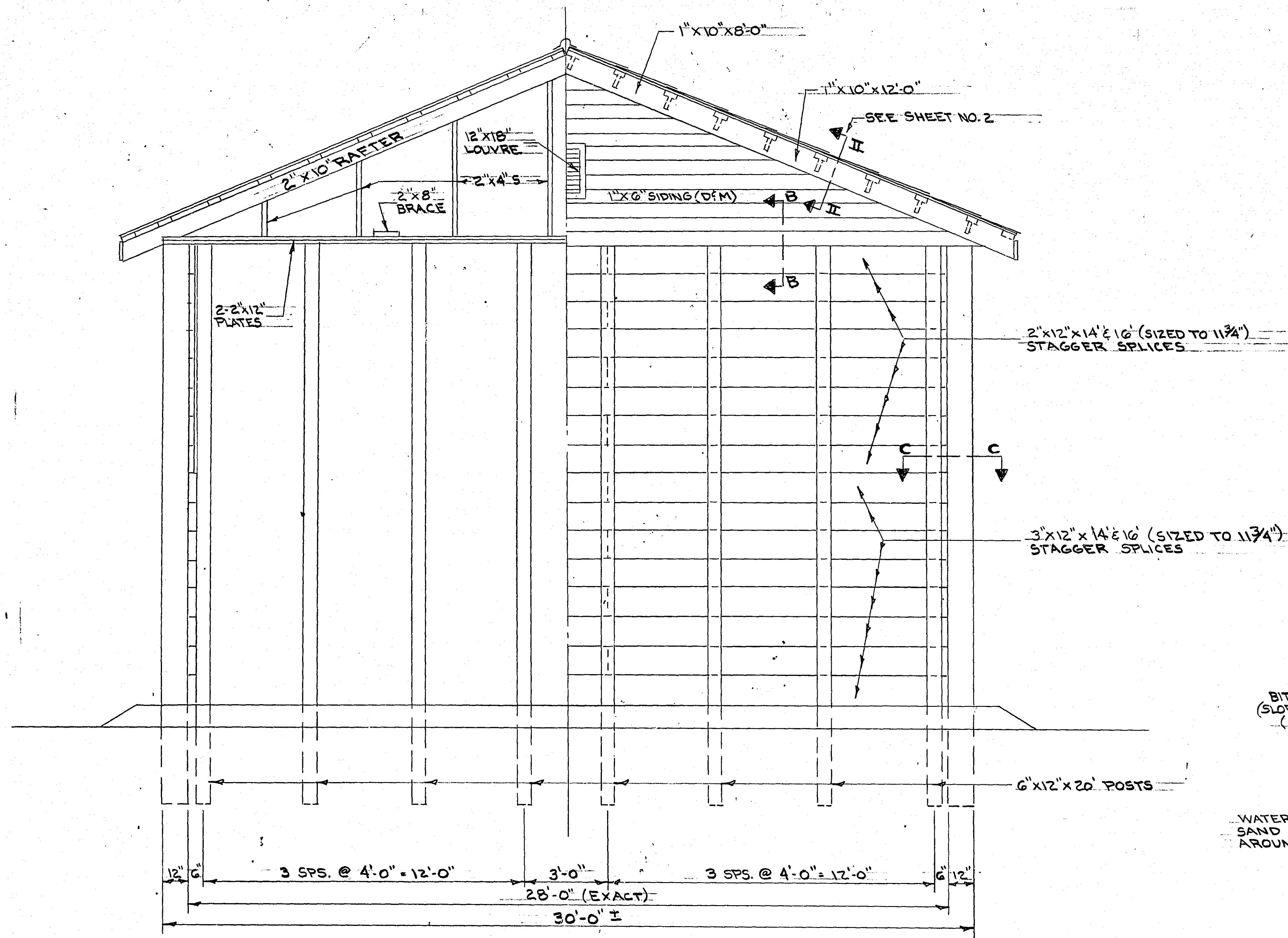
END VIEW-LOADED WALL
