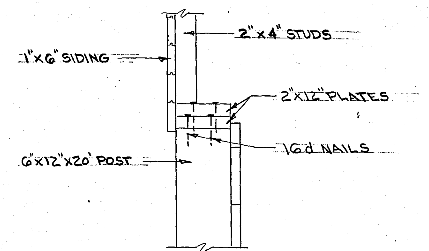
SECTION "B-B"
