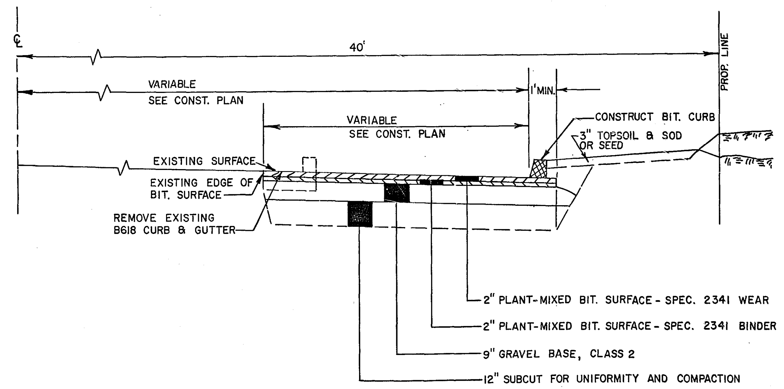
TYPICAL SECTION SILVER LAKE ROAD
