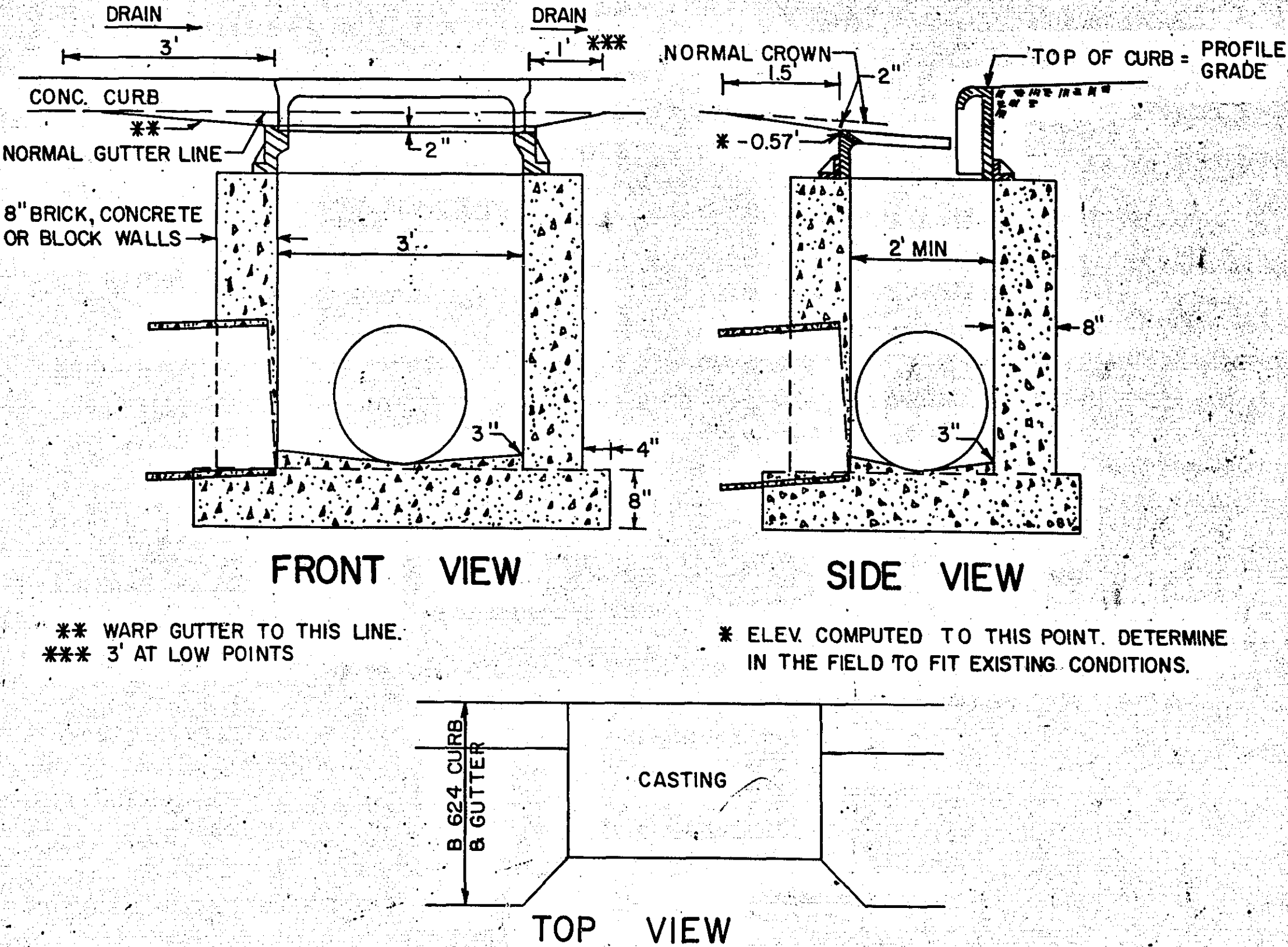
CATCH BASIN DESIGN NO. R.C.-2
