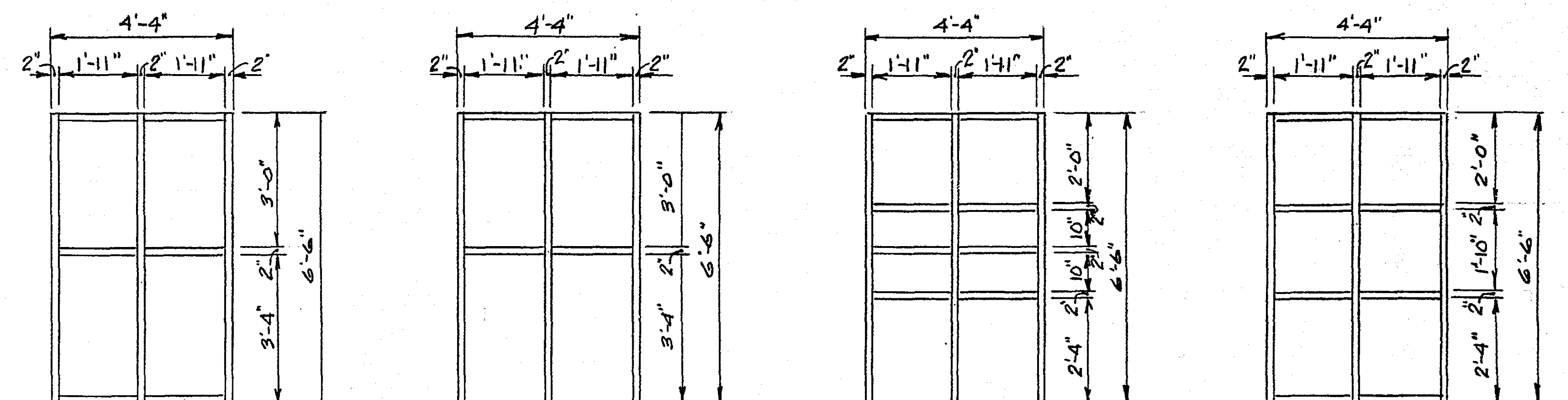
FRAMES-1 & 3
