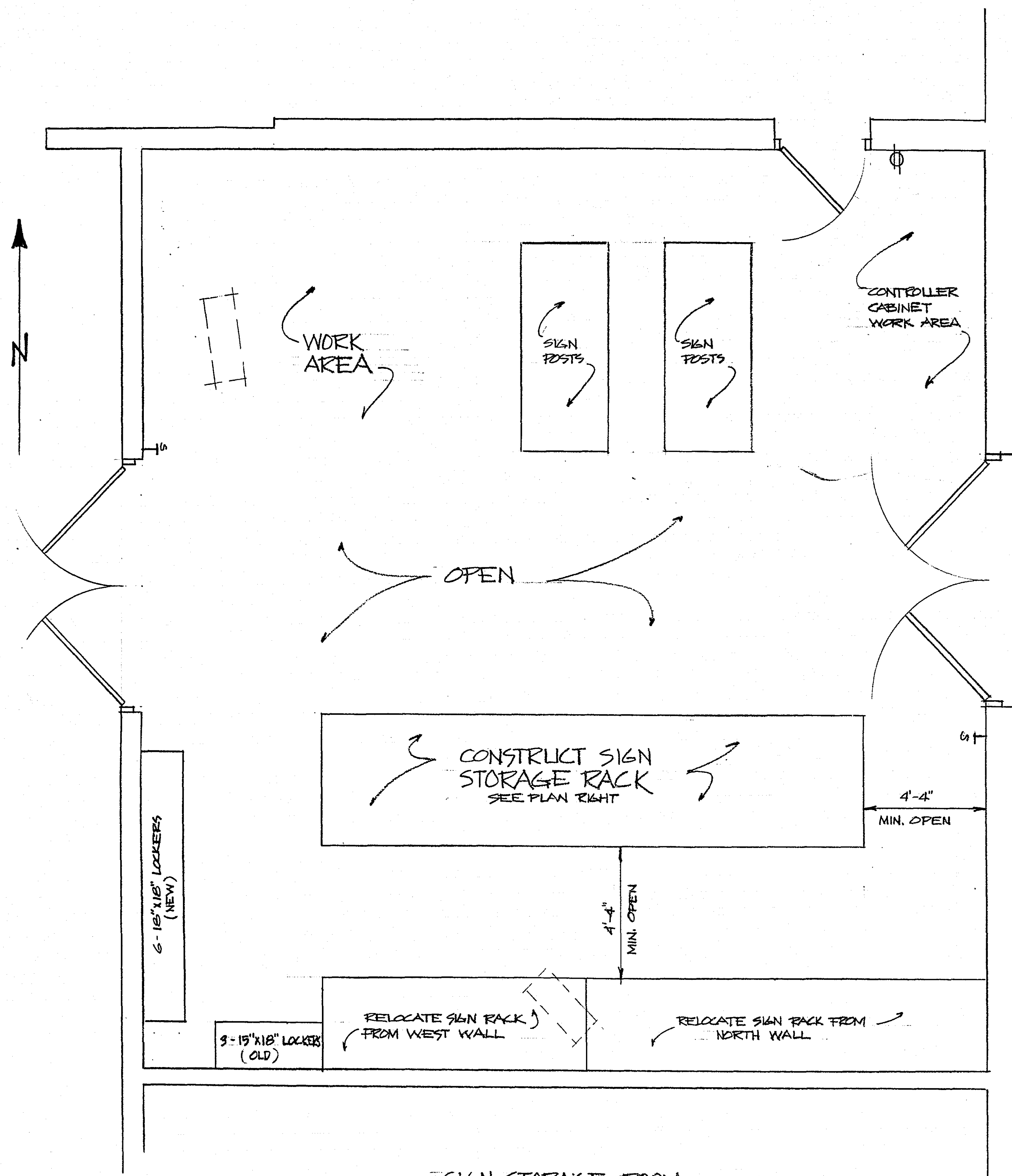
SIGN STORAGE ROOM PLAN SCALE: 3/8" = 1'-0"
