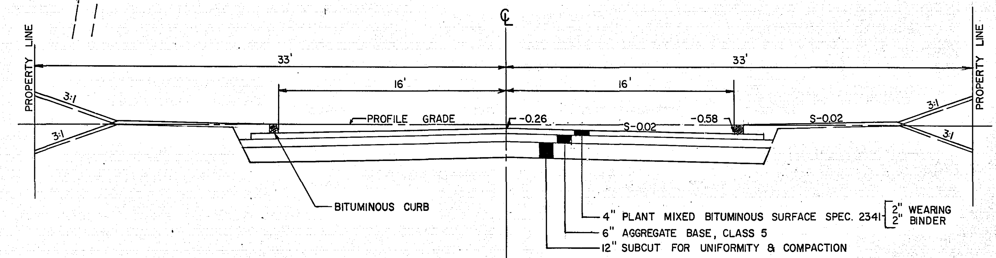
TYPICAL SECTION
