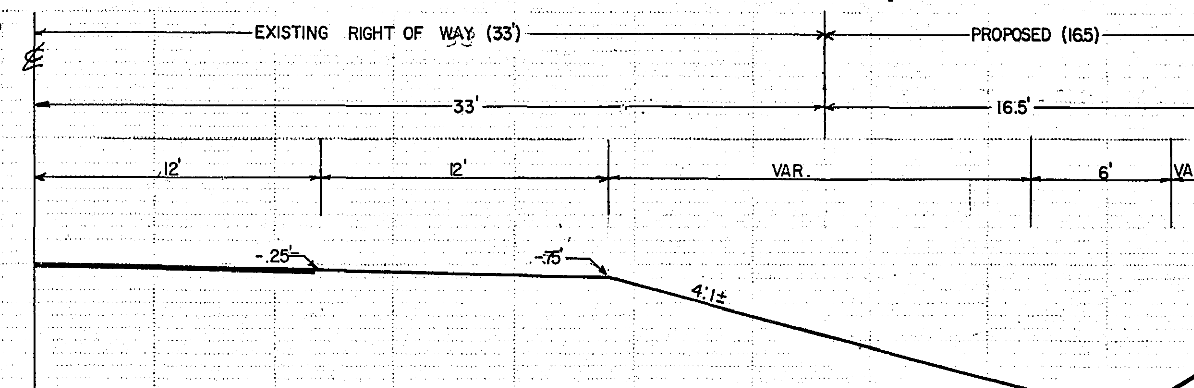
TYPICAL SECTION - EAST BOUND LANE
