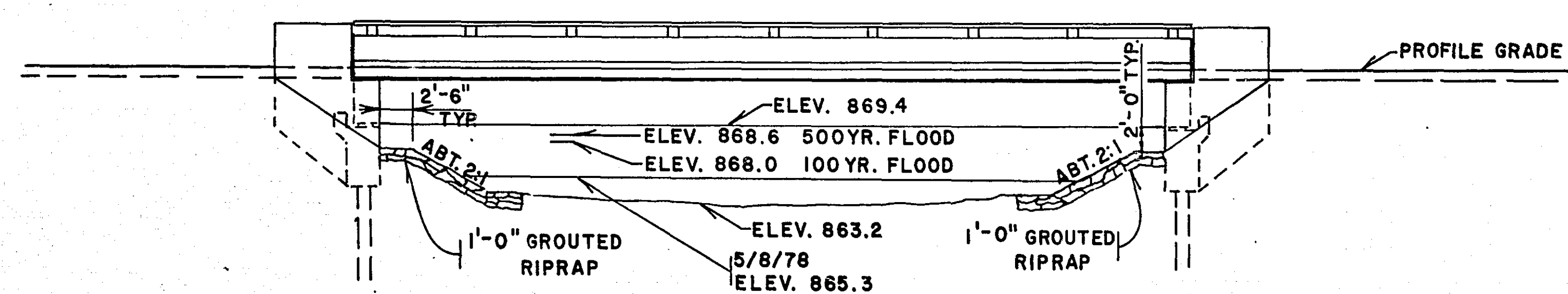
GENERAL ELEVATION \frac{3}{32}'' = 1'
