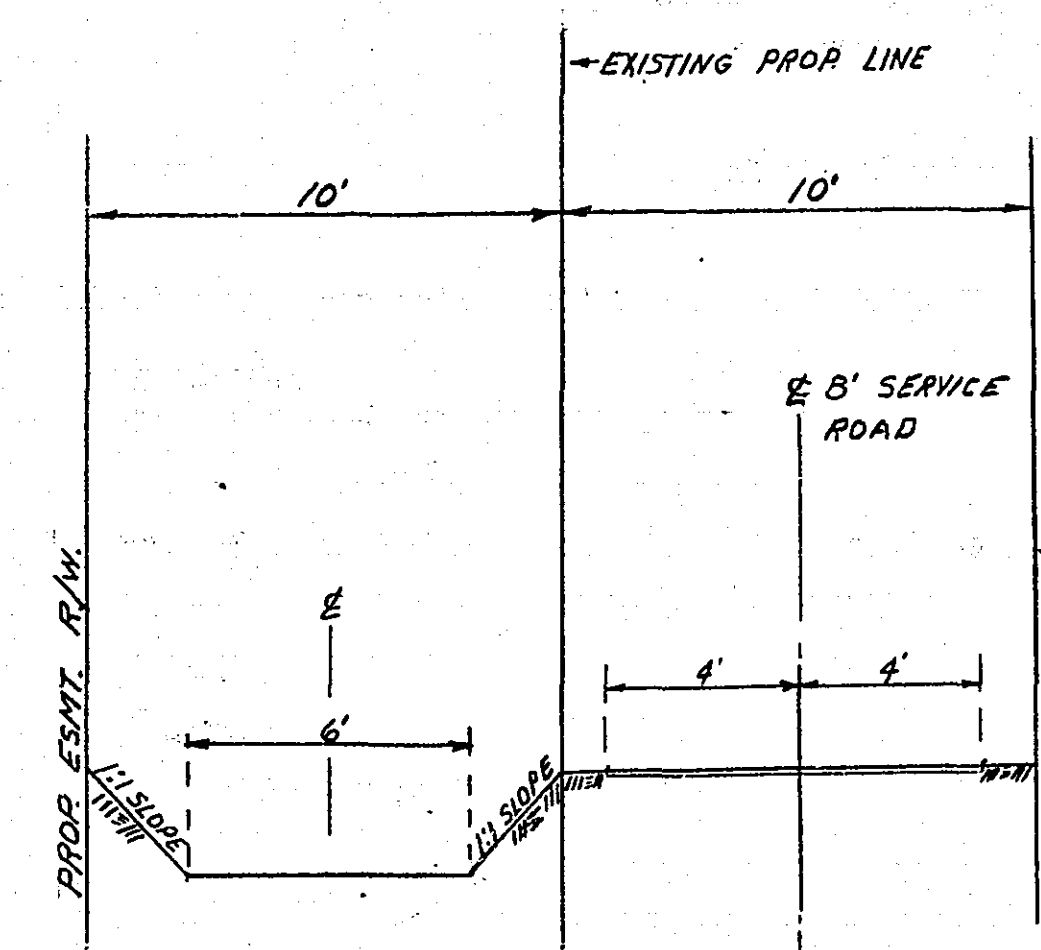
TYPICAL SECTION OF PROPOSED DITCH & SERVICE ROAD SCALE 1" = 5"
