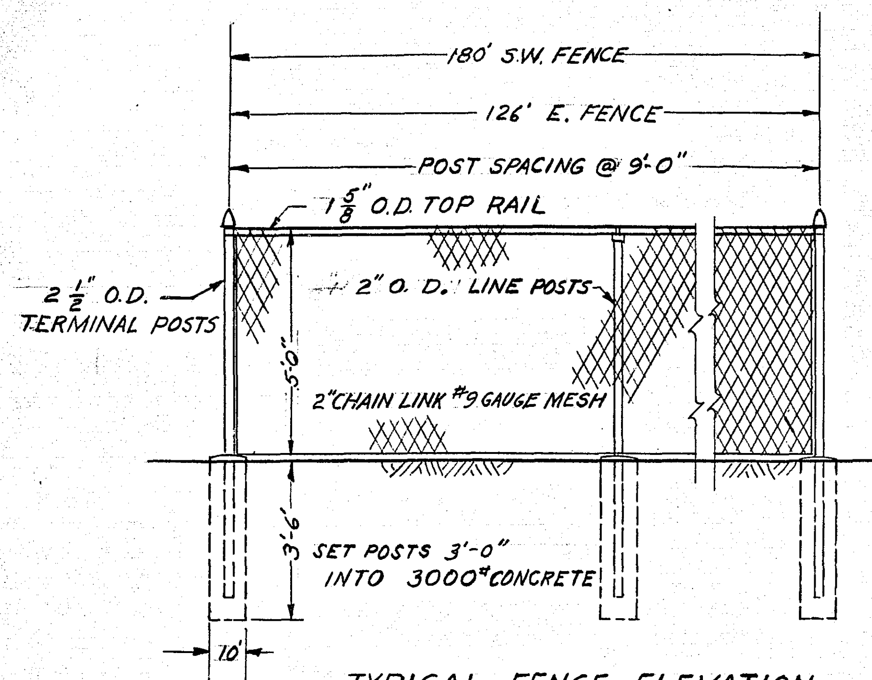
TYPICAL FENCE ELEVATION SCALE: 3/8" = 1'-0"
