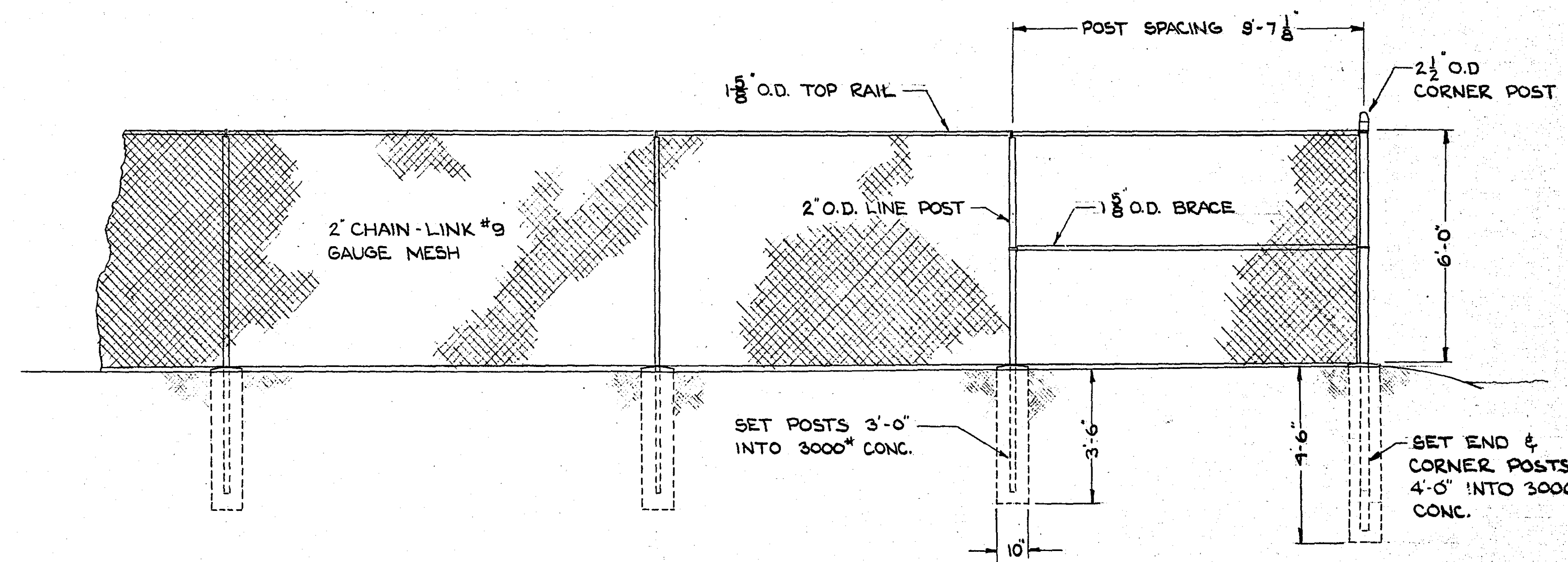
TYPICAL FENCE ELEVATION
