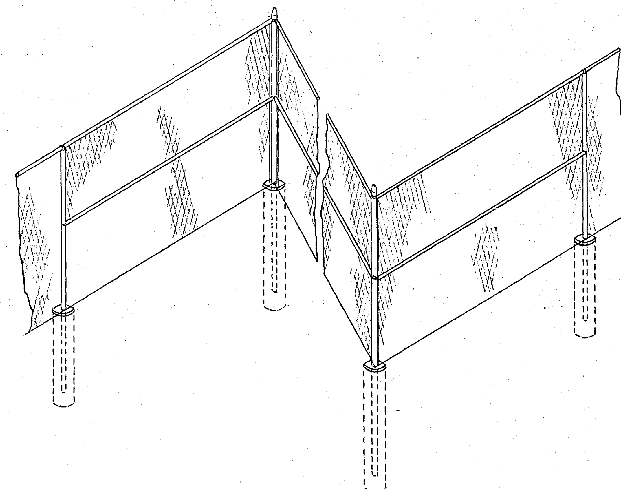
TYPICAL FENCE CORNERS
