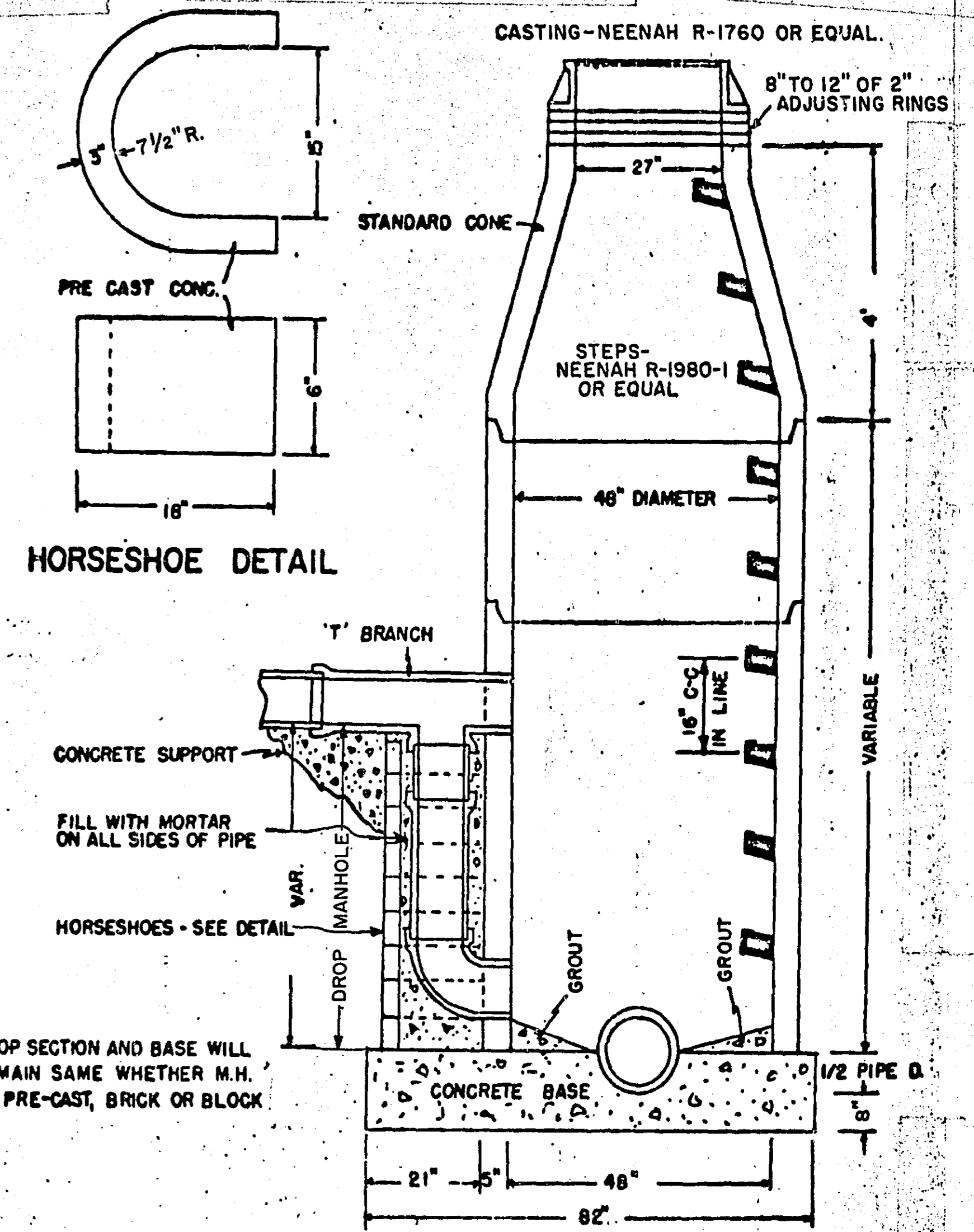
STANDARD PRECAST CONCRETE MANHOLE WITH DROP SECTION ADDED
