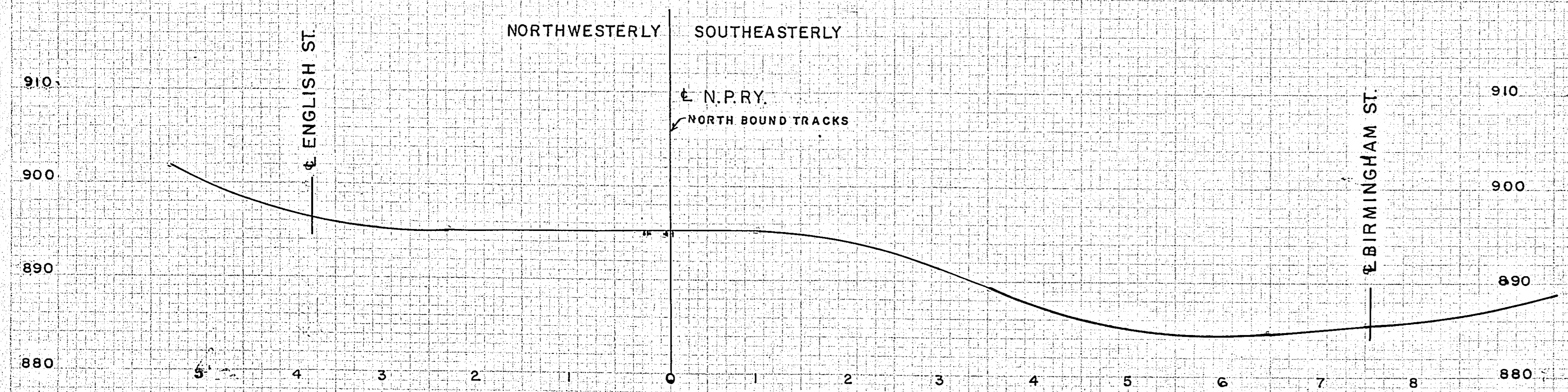
PROFILE COUNTY ROAD "B" SCALE 1" = 10' VERT. 1" = 100' HORZ.
