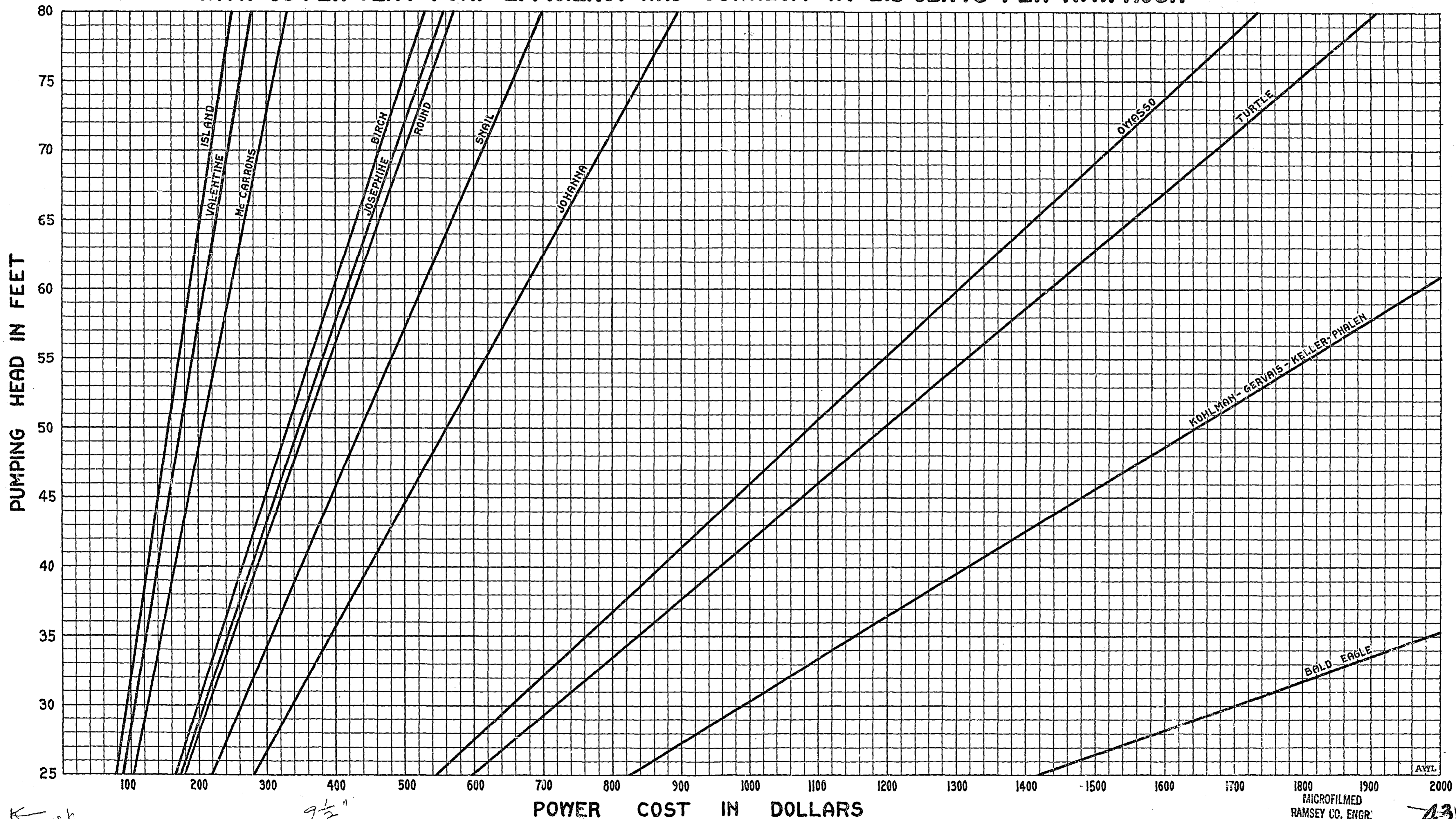
CURVES SHOWING THE COST OF PUMPING, WITH VARIOUS HEADS, THE EQUIVALENT OF ONE FOOT RISE IN ELEVATION ON RAMSEY COUNTY LAKES WHEN PUMPING 500 GAL. PER MIN. WITH 65 PER CENT PUMP EFFICIENCY AND CURRENT AT 2.5 CENTS PER K.W. HOUR
