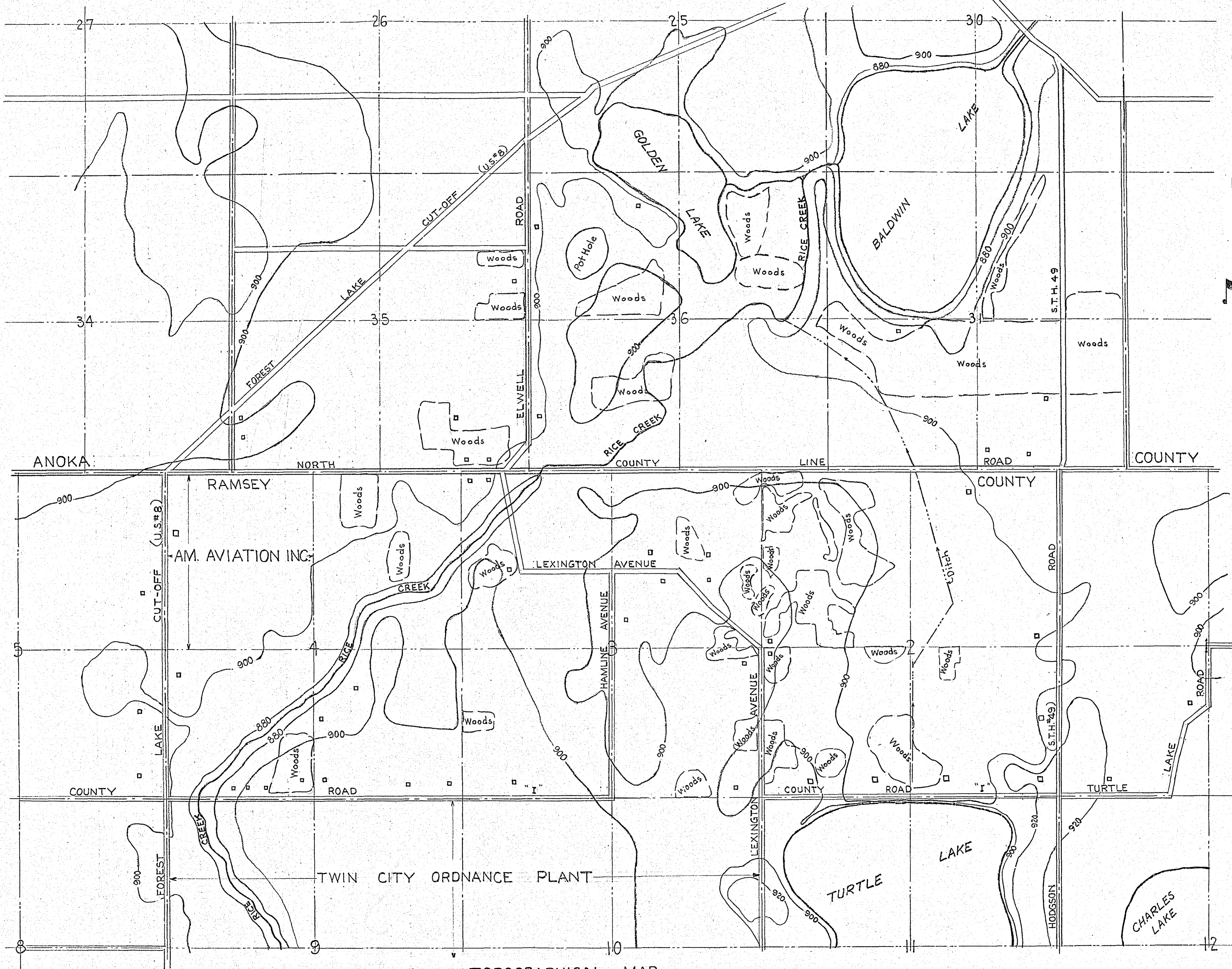
TOPOGRAPHICAL MAP OF AREA NORTH OF TWIN CITY ORDNANCE PLANT SOUTH OF U.S.HWY.8 AND WEST OF S.T.H.49 OFFICE OF RAMSEY COUNTY ENGINEER SCALE 1"=1000' MAY 1943
