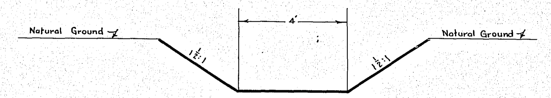
TYPICAL SECTION Note: Slopes to Conform to R/W
