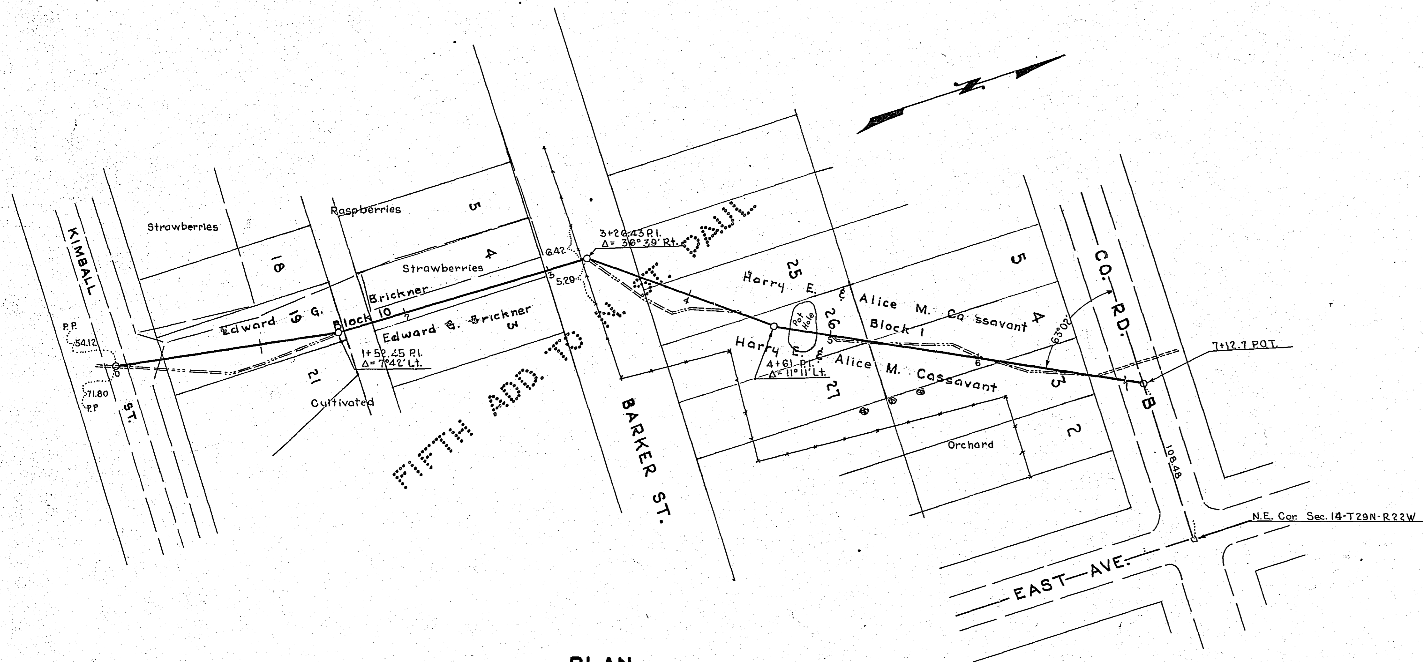
PLAN SCALE - 1" = 50'
