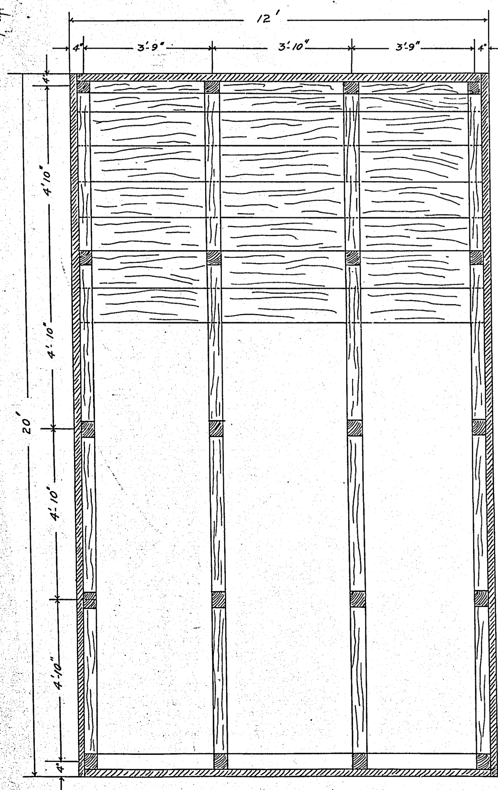
PLAN OF COAL BARGE.
