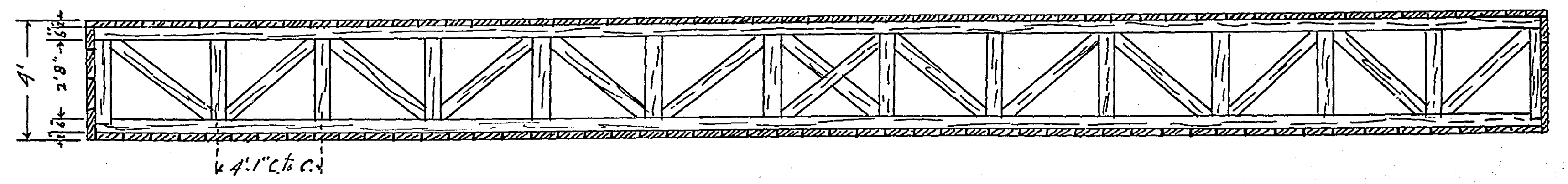
SIDE ELV. SHOWING PLANKING
