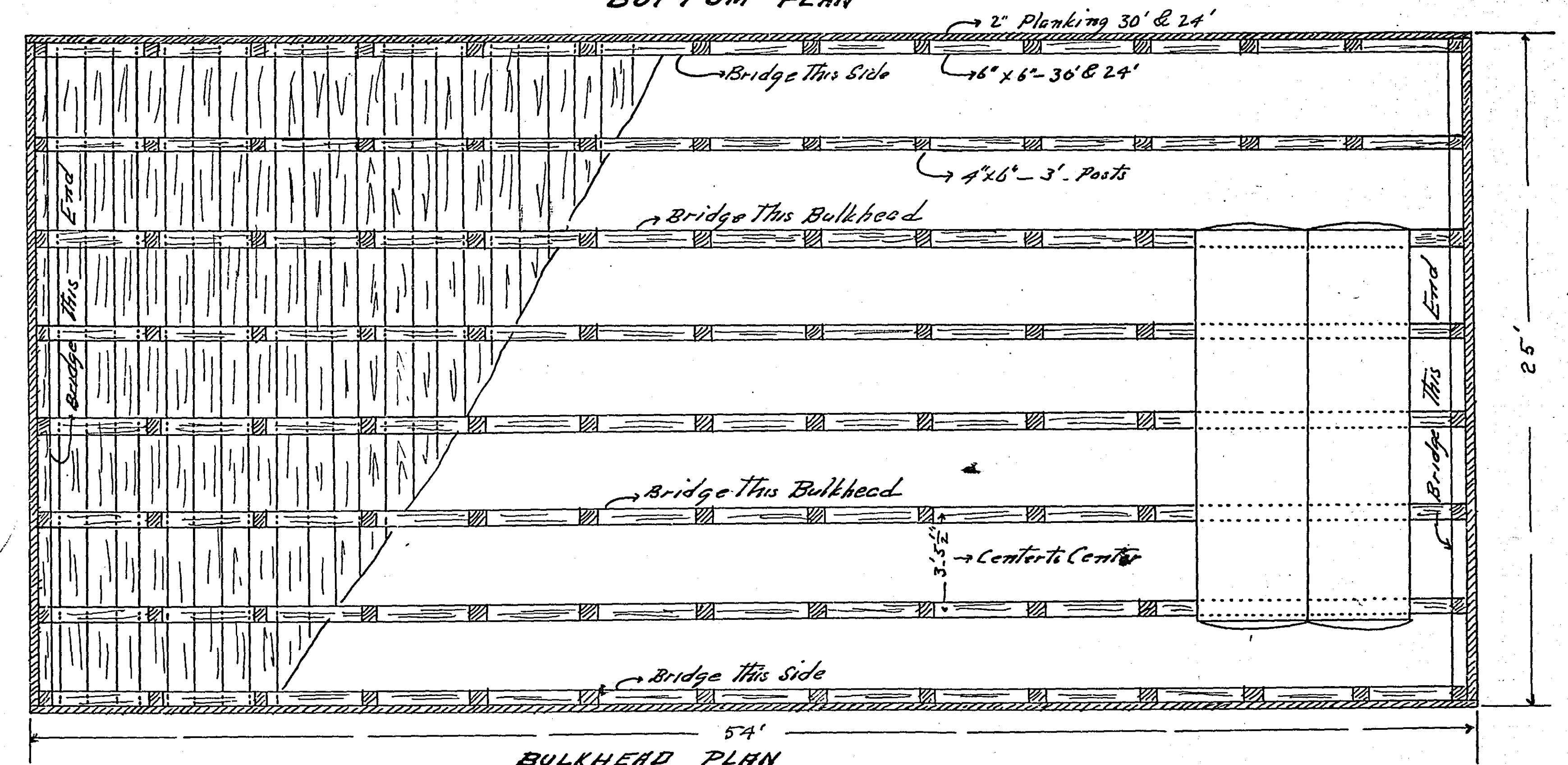
BULKHEAD PLAN
