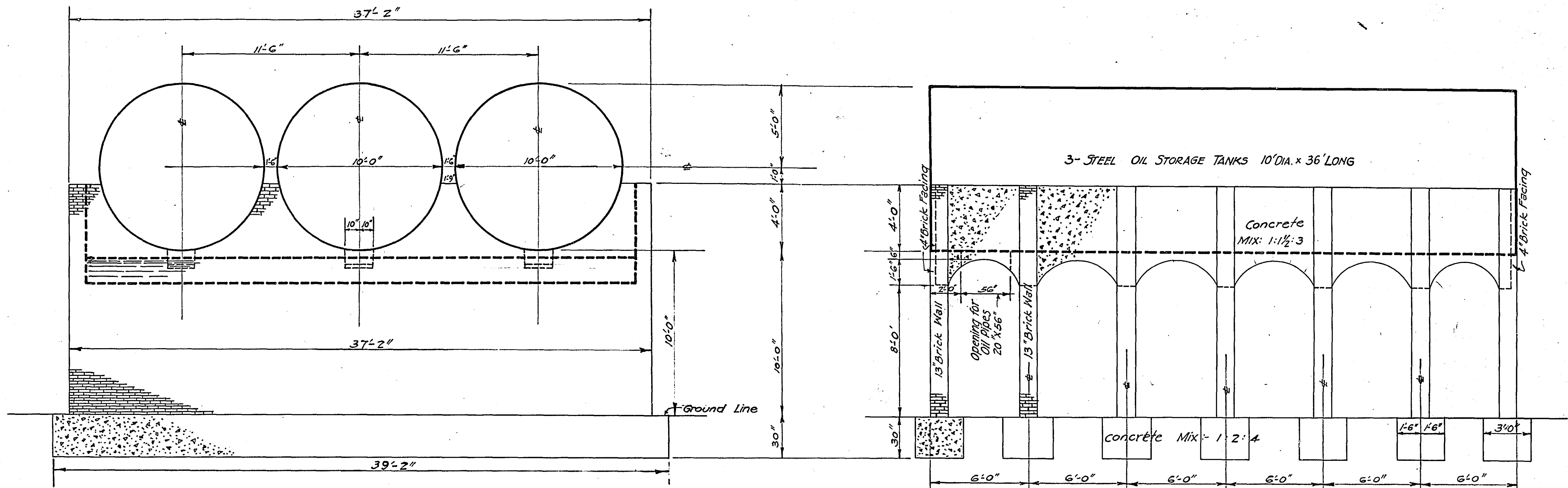
END ELEVATION OF PEDESTAL FOR OIL STORAGE TANKS
