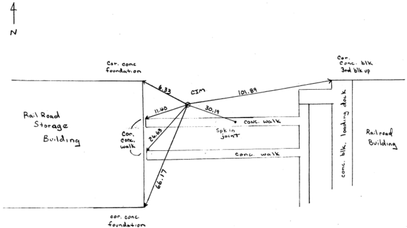
SKETCH OF REFERENCE TIES
