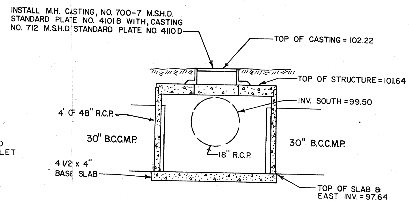
JUNCTION MANHOLE DETAIL SCALE 1"=2'
